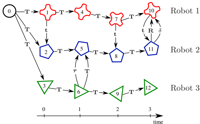
Figure 1: A time history of three robots up to time k = 3 with inter-time and inter-robot relative measurements. Each (robot, time) pair is labeled with the corresponding node index from \nu_0(3) . Arrows indicate edges in \mathcal{E}(3) , i.e., relative measurements. Each edge is labeled to indicate the type of measurement. Each robot had GPS and compass measurements at the initial time k = 0 . Thereafter, no other GPS or compass measurements were available.
