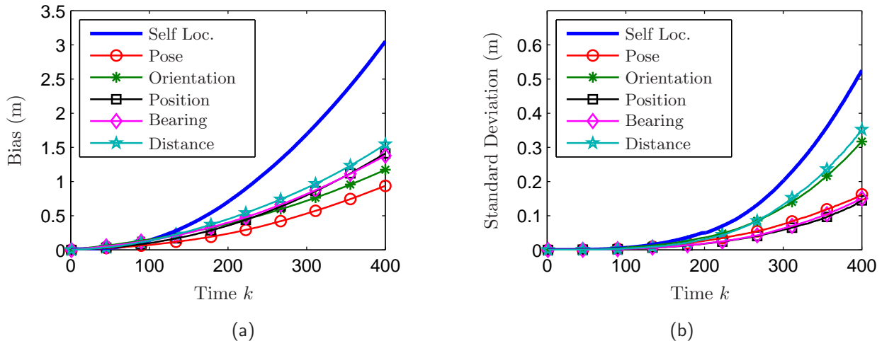
Figure 14: Experimental: The (a) bias and (b) standard deviation in position error for robot 1 with collaborative localization when both robots move in a straight line. The bias and standard deviation were empirically estimated by averaging over 24 repeated trials.
