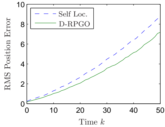
Figure 11: Simulation: The root-mean-square position error for robot 1 when the distributed algorithm is applied to a group of 5 robots utilizing inter-robot relative measurements over random paths.
