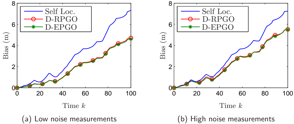
Figure 8: Simulation: comparison between D-RPGO and D-EPGO algorithms when (a) inter-robot orientation measurements are less noisy ( k = 10,000 ) and (b) inter-robot orientation measurements are more noisy ( k = 100 ) where k is the concentration parameter for the Von-Mises Fisher distribution from which the noisy measurements are drawn. The standard deviation in position estimation error of robot 1 (in a group of 5 robots utilizing noisy inter-robot relative pose measurements), computed with both algorithms, averaging over the same graph, is shown.
