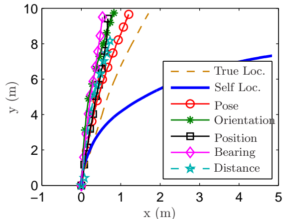
Figure 13: Experimental: A plot of the location of robot 1 in the overhead camera frame of reference when both robots move in a straight line. The true path (determined using the overhead camera), estimated path using self localization, and estimated path using the distributed collaborative localization algorithm are all reported. The various curves correspond to the type of inter-robot relative measurement used.
