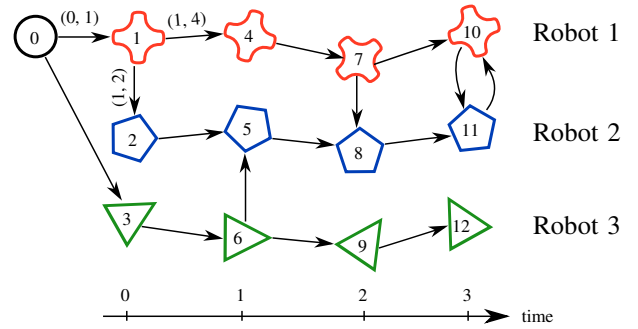
Fig. 1. A time history of three robots up to time k = 3 with inter-time and inter-robot relative pose measurements. Each (robot,time) pair is labeled with the corresponding node index from \nu_0(3) . Arrows indicate edges, i.e., relative measurements, in \mathcal{E}(3) . Robots 1 and 3 had GPS measurements at the initial time k = 0 . No other GPS measurements were available.
