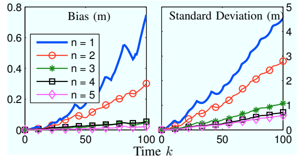
Fig. 2. The bias and standard deviation in position error for robot 1 when the distributed algorithm is applied to a group of 1, 2, 3, 4 or 5 robots.
