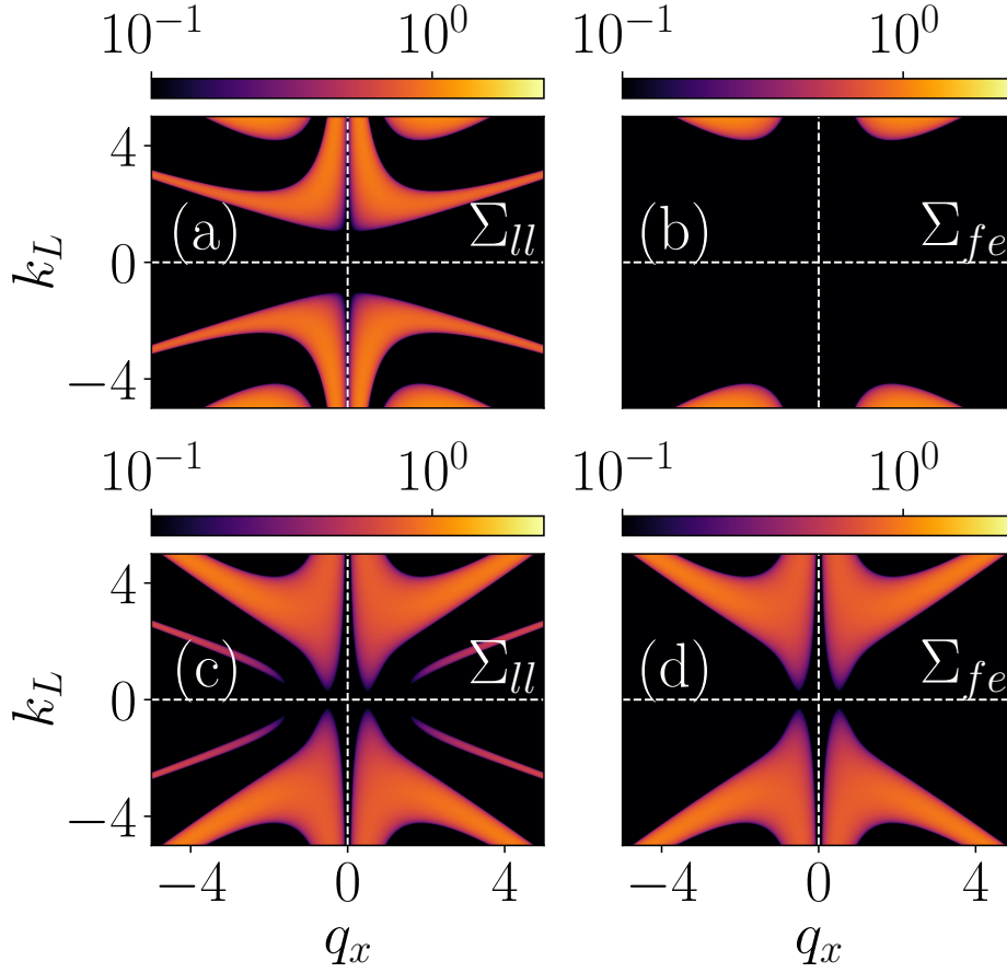
Figure 5.2: Pseudo color plot of modulational instability gain for the ferromagnetic phase ( c_0 = 5 , c_2 = -2 ) in k_L - q_x plane for (a, b) \Omega = 1 and (c, d) \Omega = -1 . Left column panel corresponds to \Sigma_{II} \equiv |\text{Im}(\omega_{II})| and right column panel corresponds to \Sigma_{fe} \equiv |\text{Im}(\omega_{fe})| . In (a), multi-band instability gain appears at k_L = 1 , and in (b) a single-band instability appears at k_L \approx 4.0 . In (c) and (d) double and single band instabilities appear at k_L > 0.25 , respectively. The second-excited branch of the eigenspectrum shows the absence of instability gain for both sets of parameters. The instability gain is symmetric about k_L and q_x .
