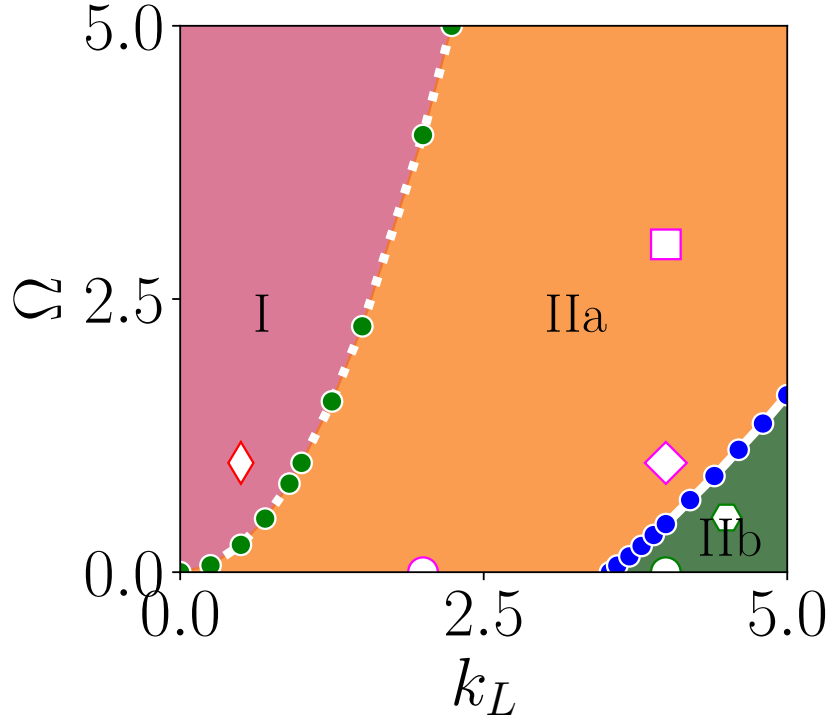
Figure 6.2: Stability phase diagram in the k_L - \Omega plane for ferromagnetic interactions ( c_0 = 50.0 and c_2 = -2.5 ) for full range of q_x with q_y = 0 . The dash-dotted white line with green dots ( k_L^2 \simeq \Omega ) separates stable (I) and unstable (II) regions. Within region II, the solid white line with blue dots ( \Omega = -1.6329 + 0.13k_L^2 ) distinguishes gapped (IIa) and gapless (IIb) spectra. The case \Omega \sim 0 lies in the unstable regime. The markers in different regions represent the coupling parameter points for which detailed collective excitation analysis is reported in the paper.
