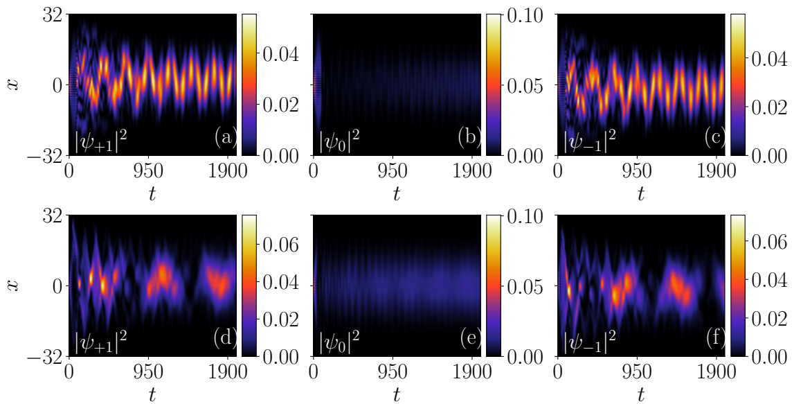
Figure 4.11: Dynamics: (a)-(c) and (d)-(f) represent the dynamics of the condensate density profile of |\psi_{+1}|^2 , |\psi_0|^2 , and |\psi_{-1}|^2 components for (k_L, \Omega) top row (3.1, 1.17), and bottom row (5.0, 2.5). The density profile holds stripe wave behavior in both cases for t < 100 and t < 50 units for the top and bottom row, respectively. Top row: t > 100 , it shows non-periodic oscillation and non-uniform density in space-time, whereas the 0-th component gets disappeared. Bottom row: t > 50 , it further gets fragmented into several small domains. This behaviour signifies the change in shape and amplitude of the density profile, along with the disappearance of the 0-th component, which confirms the dynamical instability.
