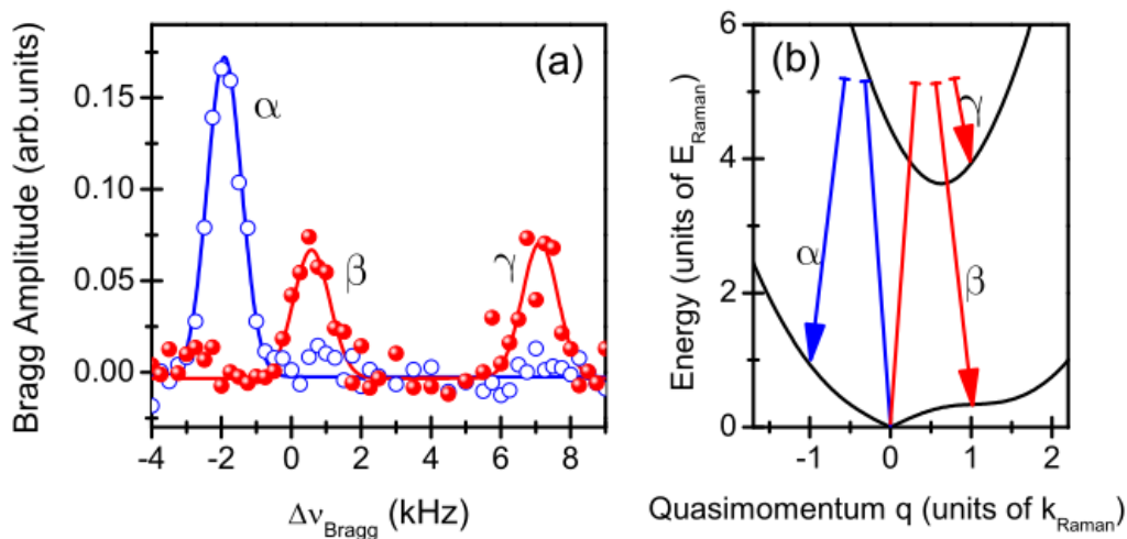
Figure 1.8: Bragg spectroscopy of a spin-orbit coupled Bose-Einstein condensate. (a) Measured Bragg response showing three resonance peaks labeled \alpha , \beta , and \gamma . (b) Schematic representation of the corresponding transitions in the Bogoliubov excitation spectrum. The \beta transition probes the finite momentum roton-like minimum. The figure is taken from Ref. [22].
