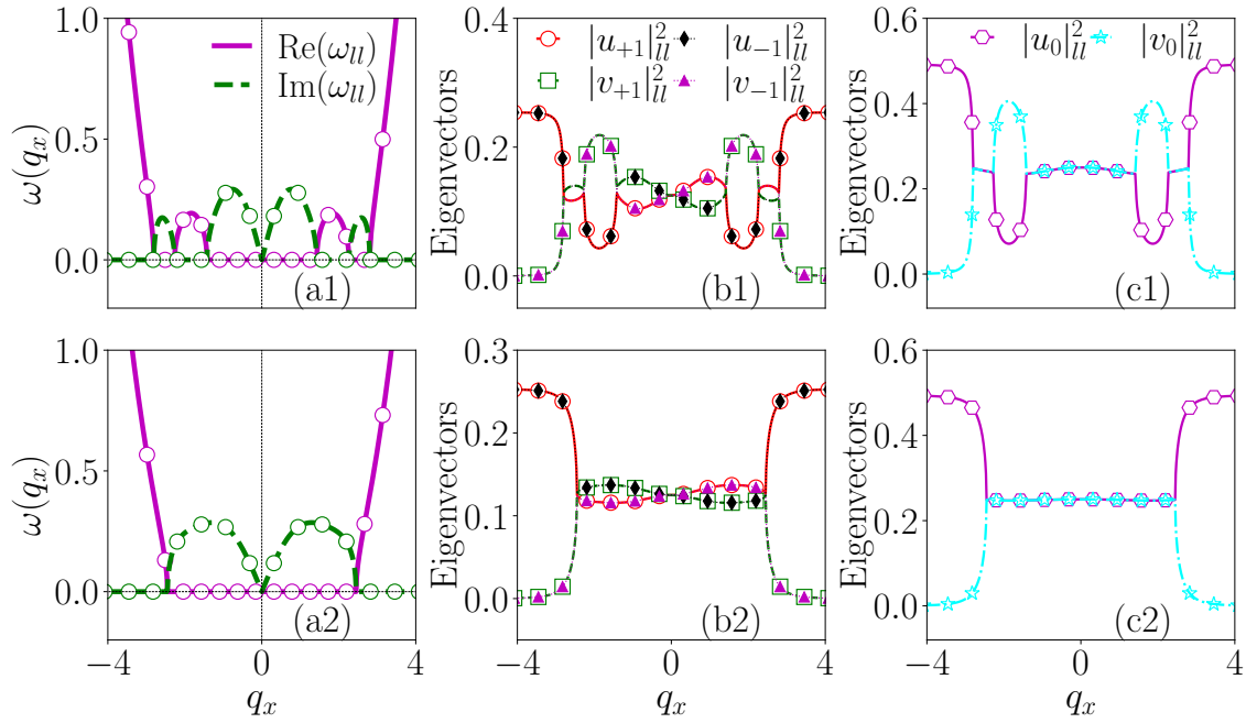
Figure 4.6: Stability excitation spectrum eigenvalues and eigenvectors: The SO and Rabi coupling strength are (k_L, \Omega) = (2.0, 2.0) (top row), and (2.35, 4.0) (bottom row), respectively. (a1), (a2) shows eigenenergy, (b1), (c1), and (b2), (c2) corresponding eigenvectors, figure labels are as like Fig. 4.3. The eigenenergy spectrum shows the presence of complex eigenfrequencies in terms of two (one) bands in the top (bottom) row, which indicates the system is dynamically unstable. Whereas the eigenvectors display the spin-dipole along with spin-like mode along the q_x momentum direction, also symmetric along the axis.
