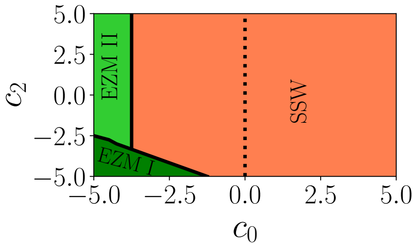
Figure 3.11: Ground state phase diagram in the c_0 - c_2 plane for fixed k_L = 3.0 , and \Omega \sim 0 . The black dotted line separates the trapless ( c_0 < 0 ) and trapped ( c_0 \gtrsim 0 ) regimes. Different quantum phases are indicated by color: green denotes the EZM I phase, lime green denotes EZM II, and coral denotes the SSW phase. For considered parameter ( k_L = 3.0, \Omega \sim 0.0 ), the system resides in the SSW phase under weak or repulsive interaction strengths, while the higher attractive strength of both c_0 and c_2 drives a transition into the EZM's phase.
