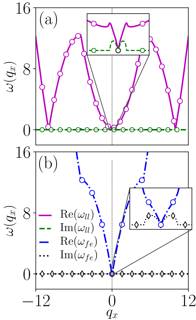
Figure 4.13: Excitation spectrum (a) low-lying and (b) first-excited branches, for the coupling strengths k_L = 5.0 , \Omega = 0.0 . The label representation is similar to the Fig. 4.9. Insets are maximized for the visualization of the complex frequency mode. Whereas the mode corresponding to the no gap between the low-lying and first excited state branch also appeared along with the symmetric roton mode.
