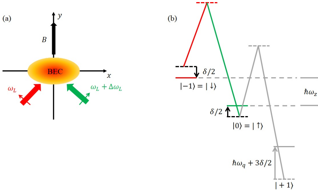
Figure 1.6: A two-photon Raman transition couples the hyperfine states |F = 1, m_F = -1\rangle and |F = 1, m_F = 0\rangle within the F = 1 ground state manifold of ^{87}\text{Rb} . The energy difference between these two states is measured by the Zeeman splitting as \hbar\omega_Z . The Raman lasers have frequency shift as \Delta\omega_L = \hbar(\omega_Z + \delta) , where \delta denotes detuning from Raman resonance. The state |F = 1, m_F = +1\rangle is shifted away in energy due to a large quadratic Zeeman shift \omega_q , effectively decoupling it from the Raman transition. This figure is adopted from Ref. [4].
