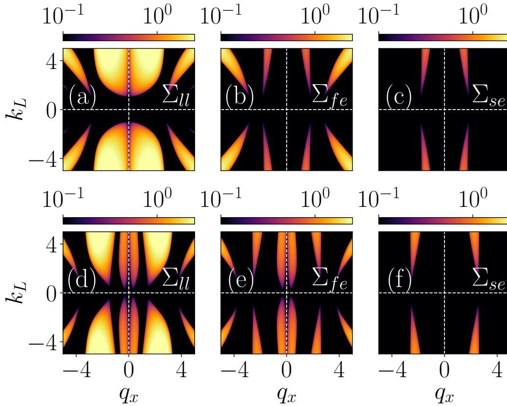
Figure 5.6: MI gain in the k_L - q_x phase plane for (a-c) \Omega = 1 and (d-f) \Omega = -1 . The interaction strengths are c_0 = c_2 = 5.0 . In the panel, the pseudo color represents similar denotations as Fig. 5.3. In the top row, we obtain the instability bands at k_L = 1.0 , following the critical relation k_L^2 = \Omega , while in the bottom row, it appears for k_L > 0.25 . Symmetry arguments are similar to Fig. 5.2.
