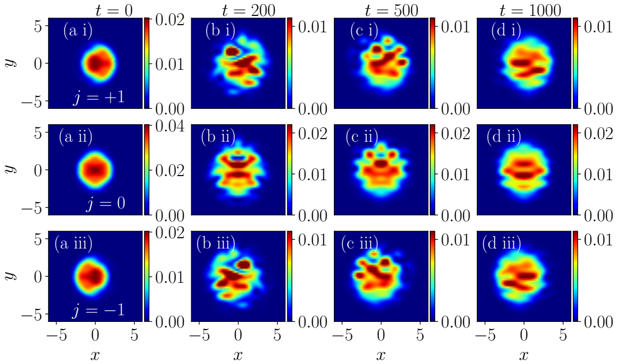
Figure 6.13: Pseudocolor plots of the stationary state and time-evolved densities. (a) The circularly asymmetric density profile of the ground state. (b–d) The density evolution at times t = 200, 500 , and 1000 , respectively. Columns (i)–(iii) correspond to the spinor components j = +1, 0 , and -1 , respectively. Parameters: lattice coupling (k_L, \Omega) = (2.0, 0.0) and interaction strengths c_0 = 50, c_2 = -2.5 .
