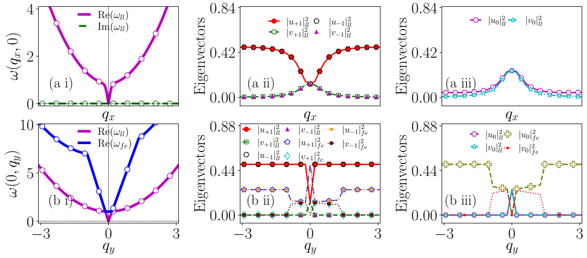
Figure 6.3: Eigenvalue spectrum and eigenvectors along the quasi-momentum directions q_x and q_y for k_L = 0.5 , \Omega = 1.0 , c_0 = 50 , and c_2 = -2.5 . Top row: low-lying branch. (a i) Eigenvalue spectrum, with \text{Re}(\omega_{ll}) (solid magenta) and |\text{Im}(\omega_{ll})| (dashed dotted green). (a ii, a iii) Corresponding eigenvector components |u_m|^2_{ll} and |v_m|^2_{ll} for m = 0, \pm 1 . Bottom row: first excited branch. (b i) Eigenvalue spectrum with \text{Re}(\omega_{fe}) (solid blue). (b ii, b iii) Corresponding eigenvector components |u_m|^2_{fe} and |v_m|^2_{fe} . All eigenvalues are real and positive, and the low-lying branch exhibits a phonon mode, indicating both dynamical and energetic stability.
