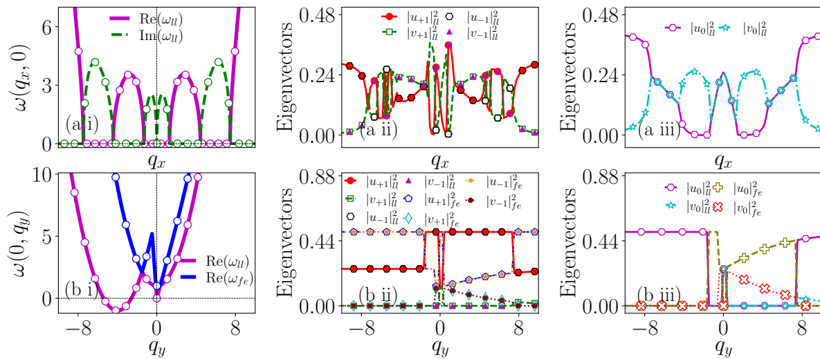
Figure 6.5: Eigenvalue spectra [(a i), (b i)] and corresponding eigenvectors [(a ii, a iii) and (b ii, b iii)] for k_L = 4.0 and \Omega = 1.0 with interaction strengths c_0 = 50.0 and c_2 = -2.5 , shown along the quasi-momentum directions q_x and q_y , respectively. Line styles and symbols follow the conventions of Fig. 6.3. A multiband instability develops along the q_x direction, leading to spin-density-spin mixed modes in the eigenvector components, while the low-lying branch exhibits negative-energy excitations along the q_y direction.
