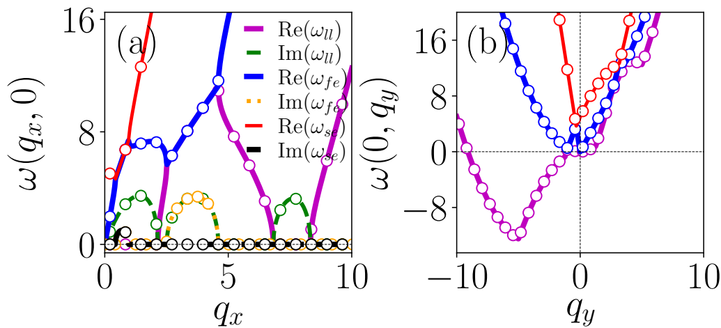
Figure 6.18: Eigenvalue spectrum along the quasi-momentum directions (a) q_x and (b) q_y . The coupling parameters are k_L = 4.0 and \Omega = 0.0 , with interaction strengths c_0 = 50 and c_2 = 2.5 . Line styles and symbols have the same meaning as in Fig. 6.14.
