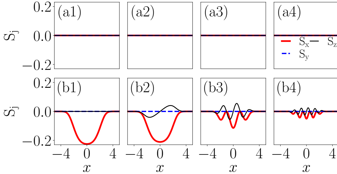
Figure 3.5: SDV component S_x , S_y , and S_z in panels (a), and (b) corresponding to the Fig. 3.4. The lines representation is the same as in Fig. 3.2. Almost zero of S_y across all phases and a single peak S_x with zero (finite) S_z , confirms the ZM (EZM I) phase for finite \Omega . All SDVs remain zero in the ZM polar phase, EZM II phase, and SSW phase for \Omega \sim 0 . Multi-peak S_x along with oscillating S_z confirms the SW phase.
