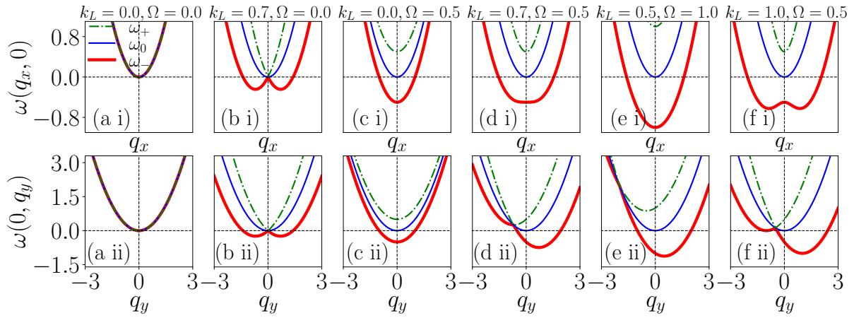
Figure 6.1: Single-particle energy spectrum top row along q_x direction and bottom row along q_y direction for the different set of SO and Rabi coupling strengths (k_L, \Omega) : (a)-(f): (0,0) , (0.7,0) , (0,0.5) , (0.7,0.5) , (0.5,1.0) , (1.0,0.5) . The thick solid red, thin solid blue line, and dash-dotted green line represent the energy eigenspectrum for \{-1,0,+1\} components of the spin, respectively. Along q_x direction, the double minimum appears in the eigenvalue dispersion, following the relation k_L^2 > \Omega , indicating the emergence of finite momentum minima, whereas for k_L^2 < \Omega the spectrum retains a single minimum at zero momentum. Along the q_y direction, the combined presence of SO and Rabi couplings produces an anisotropic dispersion with shifted minima due to symmetry breaking.
