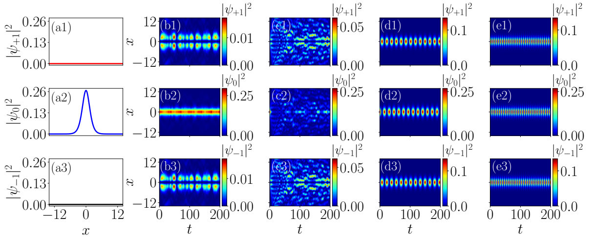
Figure 3.13: Ground state density profile (a1-a3) for m_F = +1, 0, -1 , respectively, with c_0 = -1.0 , and c_2 = 5.0 , in absence of the k_L , and \Omega . The condensate is in the ZM phase. Panels (b1-b3) and (c1-c3) depict the time evolution of the initially prepared density profile upon quenching the SO coupling from k_L \sim 0 \rightarrow 0.20 and k_L \sim 0.0 \rightarrow 1.0 , respectively. For a small quench of the SO coupling strength, periodic high-density peaks appear along the propagation direction, whereas a complex pattern emerges for stronger quench. Panels (d1-d3) and (e1-e3) exhibit the dynamics of the condensate density upon quenching the Rabi coupling \Omega \sim 0.0 \rightarrow 0.20 and \Omega \sim 0.0 \rightarrow 0.50 , respectively. In both cases, the quench of the Rabi coupling leads to the stabilization of the condensate. The SO and Rabi coupling is quenched at t = 0 units.
