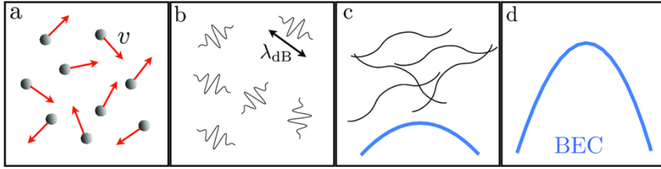
Figure 1.1: (a) Depicts particles at high temperature. (b) As the temperature decreases, the characteristic de Broglie wave length \lambda_{dB} emerges. (c) At T = T_c wavefunctions begin to overlap, and (d) Near T \approx 0 , a macroscopic wave function forms, indicating the Bose-Einstein condensate. The figure is taken from the Ref. [28].
