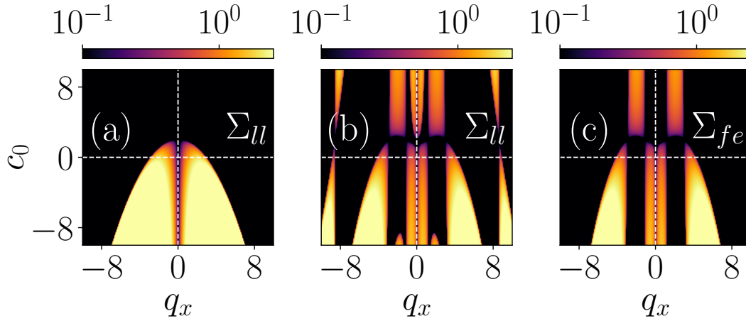
Figure 5.9: (a) Pseudo color representation of MI gain for low-lying mode \Sigma_{II} \equiv |\text{Im}(\omega_{II})| in c_0 - q_x phase plane with (k_L, \Omega) = (0.5, 1.0) . (b) and (c) represent the pseudo color representation of MI gain for low-lying mode \Sigma_{II} \equiv |\text{Im}(\omega_{II})| and first excited mode \Sigma_{fe} \equiv |\text{Im}(\omega_{fe})| respectively in the c_0 - q_x phase plane for (k_L, \Omega) = (4.5, 1.0) . The spin-exchange interaction is c_2 = -2.0 . In (a), the instability gain appears only in the low-lying branch, while in (b, c), it appears in a low-lying and first-excited branch of the excitation spectrum. In the panel, the instability gain increases upon decreasing the c_0 , showing symmetric behaviour about q_x . However, it is not symmetric about c_0 .
