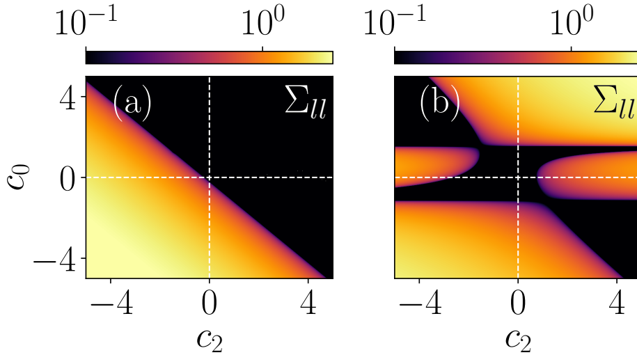
Figure 5.12: The pseudo color representation of MI gain of lowest eigen mode \Sigma_{ll} \equiv |\text{Im}(\omega_{ll})| in c_0 - c_2 phase plane for (a) (k_L, \Omega) = (0.5, 1.0) and (b) (k_L, \Omega) = (4.0, 1.0) . The quasi-momentum strength is fixed at q_x = 1 . In (a) the instability gain appears only in the low-lying branch when the total interaction strength is attractive c_0 + c_2 < 0 , while in (b) the spectrum exhibits multi-band instability. The instability gain in the eigenspectrum is neither symmetric about c_0 nor about c_2 .
