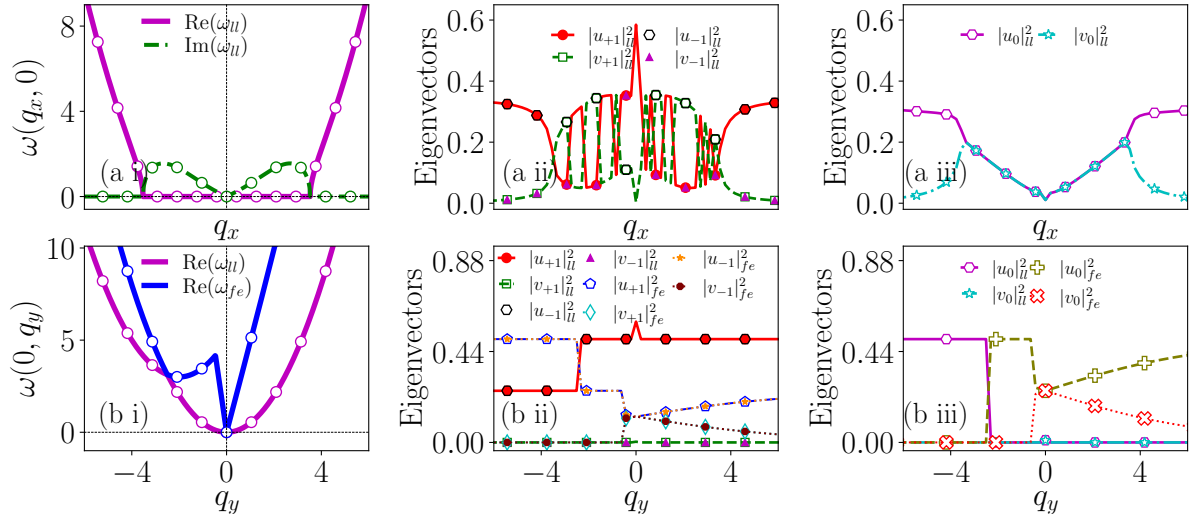
Figure 6.11: Collective excitation spectrum (a i) and (b i) with the corresponding eigenvectors (a ii, a iii) and (b ii, b iii) for k_L = 2.0 , \Omega \sim 0.0 , using interaction strengths c_0 = 50.0 and c_2 = -2.5 along with quasi-momentum directions q_x and q_y , respectively. The line styles and symbols in the top and bottom rows follow the same convention as in Fig. 6.3.
