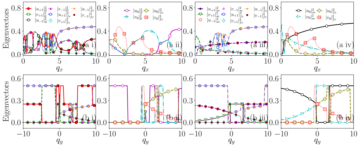
Figure 6.19: Eigenvectors corresponding to Fig. 6.18; (a i-a iv) along the quasi-momentum direction q_x , and (b i-b iv) along the quasi-momentum direction q_y . The lines and symbols have the similar meaning as in Fig. 6.15.
