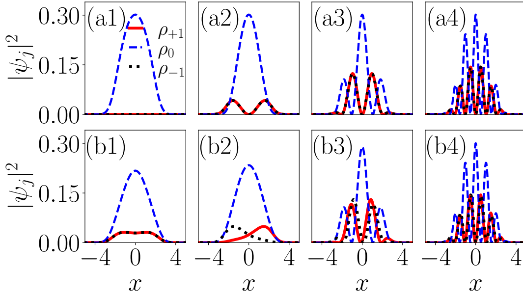
Figure 3.4: Different ground state phases of the SO coupled spin-1 BECs with antiferromagnetic interaction. Ground state density profile of the spin-component |\psi_{+1}|^2 (solid red line), |\psi_0|^2 (dashed blue line), and |\psi_{-1}|^2 (dotted black line) for (a1-a4) \Omega \sim 0.0 and (b1-b4) \Omega = 1.0 , with interaction strengths c_0 = 10 and c_2 = 5 . In each panel, k_L varies from left to right: 0.0, 0.5, 1.5, and 3.0. For \Omega \sim 0 , the ZM phase, EZM II phase, and SSW phase are observed. For finite \Omega , the SSW phase disappears, giving rise to the appearance of EZM I and SW phases.
