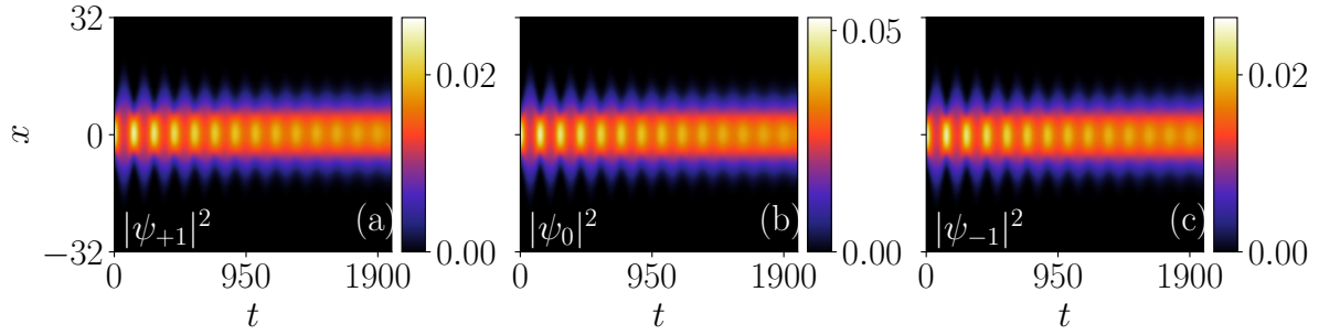
Figure 4.4: Time evolution of initially prepared stationary state density profiles illustrating dynamical stability of (a) +1 , (b) 0 , and (c) -1 components of the condensate, where the parameters are similar to Fig. 4.3. All three components |\psi_{+1}|^2 , |\psi_0|^2 , and |\psi_{-1}|^2 depict stable breather-like dynamics, which validate the dynamical stability of the condensate.
