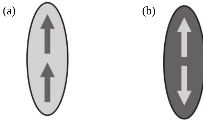
Figure 1.3: Magnetic phases of spin-1 Bose-Einstein condensates (a) c_2 < 0 : ferromagnetic phase, and (b) c_2 > 0 : antiferromagnetic phase. The figure is adopted from the Ref. [35].
