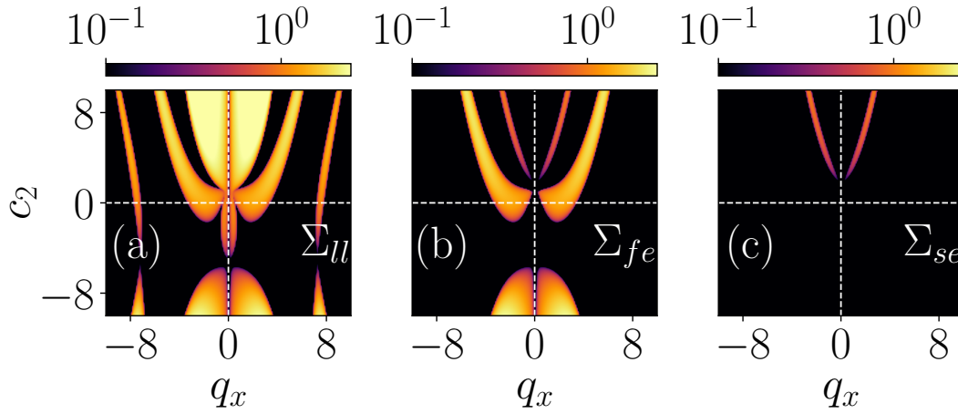
Figure 5.11: MI in c_2 - q_x phase plane for (a-c) k_L = 4.0, \Omega = 1.0 , with c_0 = 5.0 . The pseudo color bar is similar to Fig. 5.3. The instability gain of the spectrum increases upon increasing c_2 , showing the symmetric behaviour about q_x . However, it is not symmetric about c_2 .
