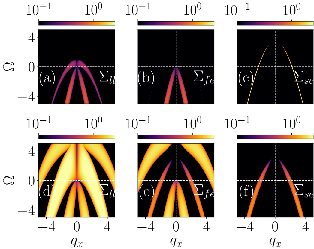
Figure 5.7: MI gain in \Omega - q_x phase diagram for (a-c) k_L = 1 , and (d-f) k_L = 4.0 . Here, the density-density interaction, c_0 = 5.0 , and spin-dependent interaction c_2 = 5.0 . The pseudo-color bar in the figure is similar to Fig. 5.3. Multi-band instability appears for the low-lying and first-excited branches of the spectrum, while the second-excited branch shows single-band instability. The instability gain appears is not symmetric about \Omega and increases upon decreasing the \Omega . However, it shows symmetric behaviour about q_x .
