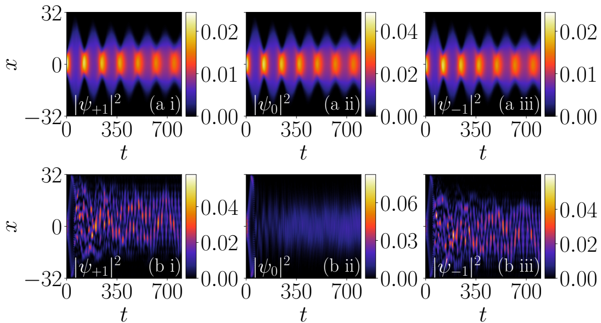
Figure 5.14: Time evolution of the condensate in x - t plane for |\psi_{+1}|^2, |\psi_0|^2, |\psi_{-1}|^2 components of the condensate for (top row) (k_L, \Omega) = (0.5, 1.0) , and (bottom row) (k_L, \Omega) = (4.5, 1.0) , upon quenching the trap strength to one-third of its initial value. The interaction strengths are c_0 = 5.0 and c_2 = -2.0 . In the top row, the density profile shows stable behaviour throughout, showing the dynamical stability of the condensate. In the bottom row, the density profile holds its SW nature for a while; at a later time, |\psi_{\pm 1}|^2 fragments in small domains and show decay in amplitude while the zeroth component diminishes at first, further gains the amplitude.
