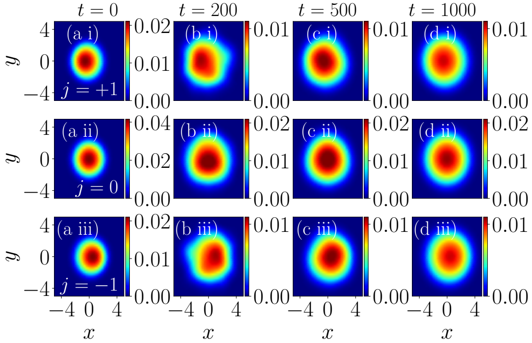
Figure 6.4: Pseudocolor density plots showing the time evolution of the condensate following a quench of the harmonic trap strength from \lambda = 1 to \lambda = 0.5 . Panel (a) shows the ground-state density profile, while panels (b-d) correspond to the evolution at t = 200, 500 , and 1000 , respectively, for coupling parameters (k_L, \Omega) = (0.5, 1.0) and interaction strengths c_0 = 50, c_2 = -2.5 . Columns (i-iii) represent the j = +1, 0, -1 components of the spinor condensate. The persistence of the density profiles over long times demonstrates the dynamical stability of the condensate under the trap quench.
