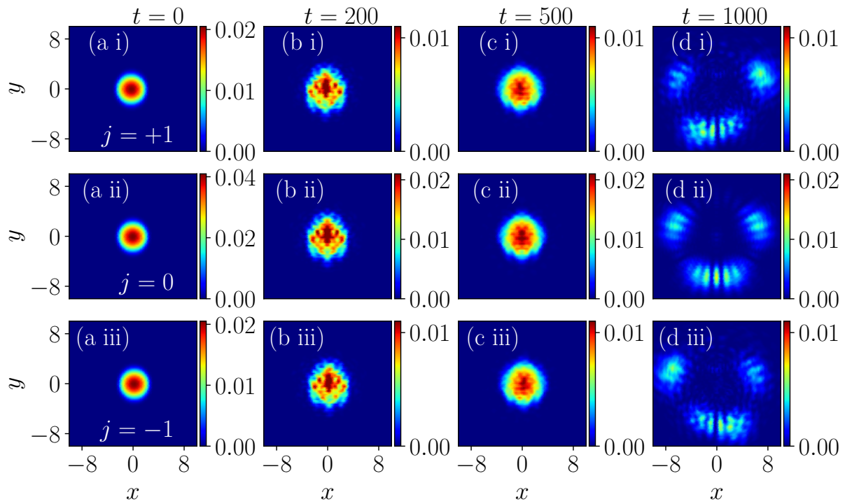
Figure 6.8: Pseudocolor density plots showing the time evolution of the condensate following a quench of the harmonic trap strength from \lambda = 1 to \lambda = 0.5 . (a) Stationary state density profile. (b-d) snapshots during time evolution at t = 200, 500, 1000 , respectively, for coupling parameters (k_L, \Omega) = (4.0, 1.0) , with interaction strengths c_0 = 50, c_2 = -2.5 . Each column represents the spinor components, with j = +1 (top), 0 (middle), and -1 (bottom).
