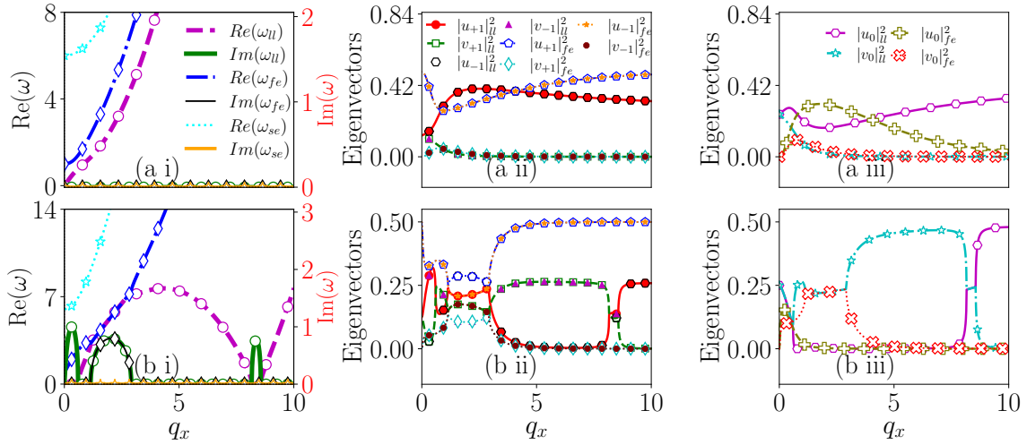
Figure 5.1: Eigenvalue and corresponding eigenvectors for (a) (k_L, \Omega) = (0.5, 1.0) showing real eigenfrequencies and (b) (k_L, \Omega) = (4.5, 1.0) showing the multiband instability for ferromagnetic interaction c_0 = 5 , c_2 = -2.0 . The dashed magenta line represents \text{Re}(\omega_{II}) , the thick green line represents |\text{Im}(\omega_{II})| , dash-dotted blue line represents \text{Re}(\omega_{fe}) , the solid black line represents |\text{Im}(\omega_{fe})| , dotted cyan line represents \text{Re}(\omega_{se}) , and the solid orange line represents |\text{Im}(\omega_{se})| , here solid and dash-dotted lines are the analytical results of BdG Eq. 5.8 and open circles are numerical results obtained by solving Eq. 5.5. Eigenvectors of low-lying branch are |u_{+1}|_{II}^2 (red dot), |u_{-1}|_{II}^2 (black hexagons), |u_0|_{II}^2 (magenta hexagons), |v_0|_{II}^2 (cyan open stars), |v_{+1}|_{II}^2 (green open squares), and |v_{-1}|_{II}^2 (magenta triangles). For the first-excited branch, |u_{+1}|_{fe}^2 (blue open pentagon), |u_{-1}|_{fe}^2 (orange stars), |u_0|_{fe}^2 (olive open plus), |v_0|_{fe}^2 (red open x with the dotted line), |v_{+1}|_{fe}^2 (cyan open diamond), and |v_{-1}|_{fe}^2 (maroon dots). (a i) exhibits only real eigenfrequencies, and (b i) depicts multi-band instability, which is symmetric in the quasi-momentum direction. Corresponding eigenvectors depict density-like mode and spin-like mode, respectively. The UAC among branches results in I_0 type instability band in the eigenspectrum. The vertical scale on the right represents the magnitude of imaginary eigenfrequencies.
