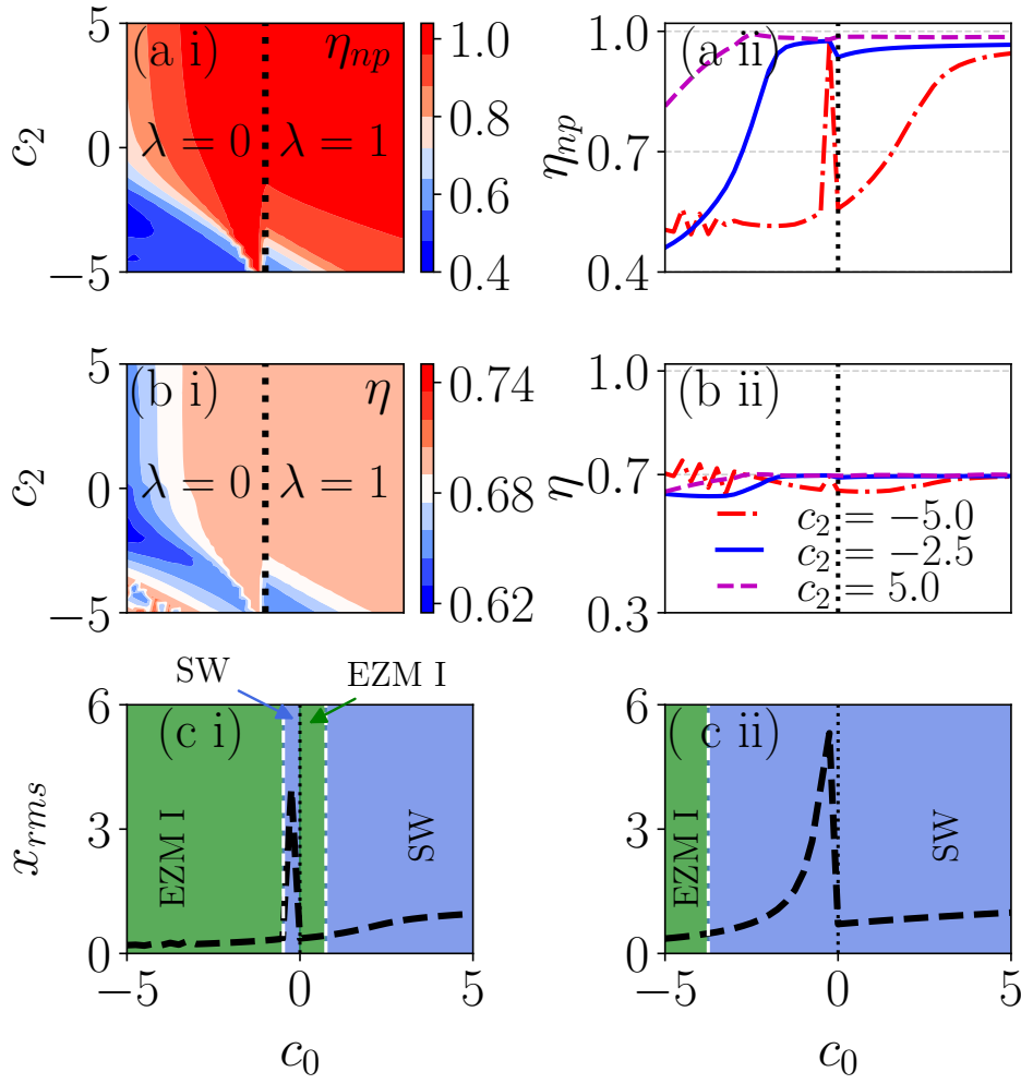
Figure 3.9: Miscibility parameters (a) \eta_{np} and (b) \eta as functions of interaction strengths c_0 and c_2 , for fixed k_L = 3.0 and \Omega = 1.0 . In (a i), and (b i), both c_0 and c_2 are varied within the range [-5, 5] . (a ii), and (b ii) show \eta_{np} and \eta as functions of c_0 for fixed values of c_2 = -5.0 (dash-dotted red line), -2.5 (solid blue line), and 5.0 (dashed magenta line). Panels (c i) and (c ii) depict the root-mean-square size x_{rms} of the condensate for c_2 = -5.0 and c_2 = 5.0 , respectively, as c_0 is varied. The background color shading represents distinct quantum phases: green indicates the EZM I phase and blue indicates the SW phase, highlighting the phase transition of the condensate. The black dotted line indicates the boundary separating trapped regime ( c_0 \gtrsim 0 ) and untrapped regime ( c_0 < 0 ) condensates.
