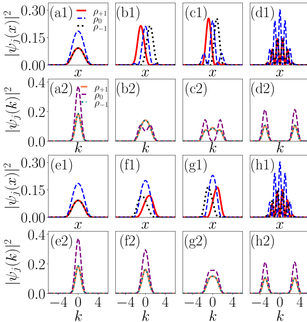
Figure 3.1: Different ground state phases of the SO coupled spin-1 BECs with ferromagnetic interaction. Real-space (top) and momentum-space (bottom) density profiles of spin components |\psi_{+1}(x)|^2 (solid red), |\psi_0(x)|^2 (dashed blue), and |\psi_{-1}(x)|^2 (dotted black), along with their corresponding momentum-space densities |\psi_{+1}(k)|^2 (solid coral), |\psi_0(k)|^2 (dashed purple), and |\psi_{-1}(k)|^2 (dotted green), under varying Rabi coupling \Omega and spin-orbit coupling k_L . Interaction strengths are fixed at c_0 = 10 and c_2 = -5.0 . Panels (a-d) correspond to \Omega \sim 0 and panels (e-h) to \Omega = 1.0 , with k_L = 0.0, 1.0, 1.5, 3.0 increasing from left to right in each set. For \Omega \sim 0 , increasing k_L induces transitions through ZM, EZM I, SW, and SSW ground state phases. At finite \Omega , the SSW phase is absent.
