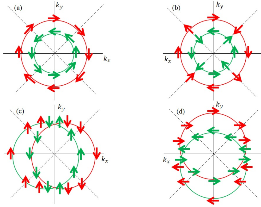
Figure 1.5: Spin textures associated with different spin-orbit coupling configurations. Panels (a) and (b) illustrate two-dimensional spin-orientations. (a) Rashba coupling, proportional to \lambda_R \times (k_y\sigma_x - k_x\sigma_y) arising from structural inversion symmetry (b) Dresselhaus coupling, proportional to \lambda_D \times (-k_y\sigma_x - k_x\sigma_y) , originating from bulk inversion symmetry. Panels (c) and (d) depict effective one-dimensional SO couplings obtained when Rashba and Dresselhaus couplings contribute equally, producing two distinct unidirectional forms: (c) -\lambda_{RD}k_x\sigma_y and (d) \lambda_{RD}k_y\sigma_x . The red and blue colors represent the different spins. This figure is adopted from Ref. [43]
