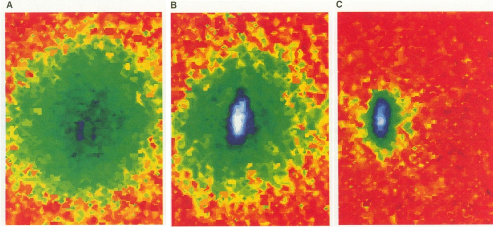
Figure 1.2: False color images depict the cloud's velocity distribution at three stages: (A) immediately before the condensate forms, (B) just after it appears, and (C) after additional evaporation produces nearly a pure condensate. The round shape of the non-condensate fraction (mostly yellow and green) reflects an isotropic velocity distribution, consistent with thermal equilibrium. In contrast, the condensate fraction (mostly blue and white) has an elliptical shape, indicating a strongly non-thermal distribution. The figure is taken from Ref. [14].
