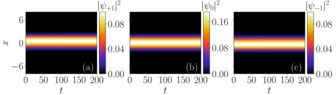
Figure 2.2: Stability of the condensate density profile during real-time propagation for (a) |\psi_{+1}|^2 , (b) |\psi_0|^2 , and (c) |\psi_{-1}|^2 . To obtain the ground state, we consider k_L = 0.5 , \Omega = 1.0 , c_0 = 10 , and c_2 = -5.0 . The density profile remains unchanged in both shape and amplitude during time evolution, indicating the stable nature of its ground state.
