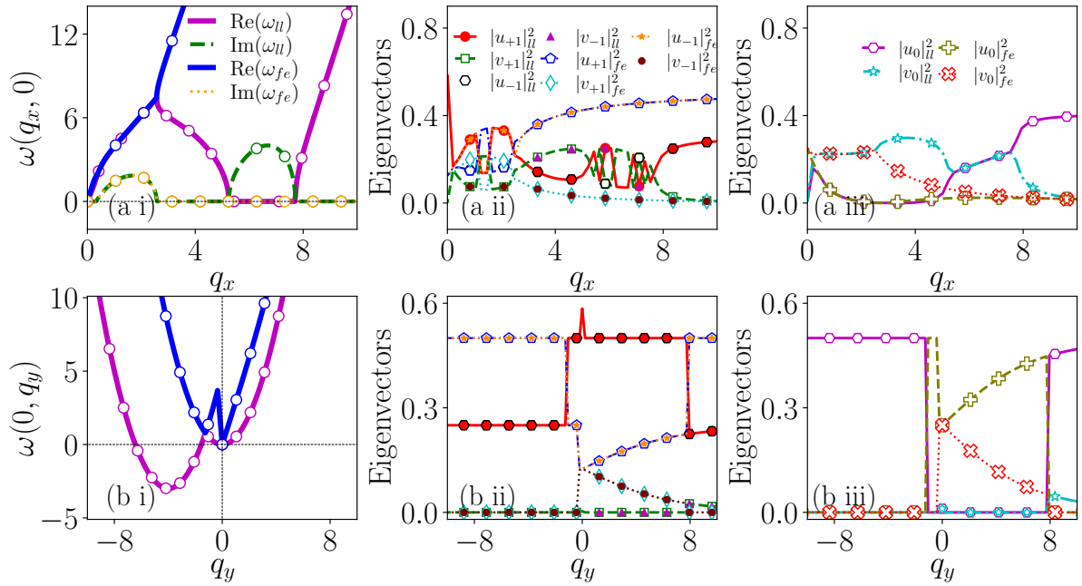
Figure 6.12: (a i, b i) Eigenvalue spectrum and (a ii, a iii, b ii, b iii) corresponding eigenvectors for k_L = 4.0 in the static limit ( \Omega = 0 ), with interaction strengths c_0 = 50.0 and c_2 = -2.5 . The spectra and eigenvectors are plotted as functions of the quasi-momenta q_x and q_y , respectively. The line styles and symbols in the top and bottom rows follow the same convention as in Fig. 6.9.
