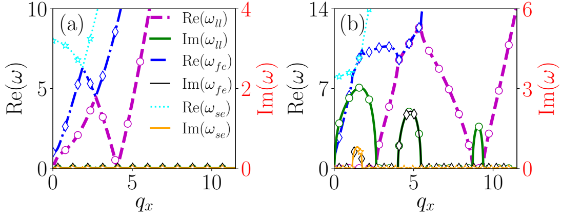
Figure 5.4: Eigenspectrum with antiferromagnetic interaction ( c_0 = 5.0 , c_2 = 5.0 ) for (a) (k_L, \Omega) = (0.5, 1.0) , and (b) (k_L, \Omega) = (4.5, 1.0) . The lines and symbols representation is same as in Fig. 5.1(a i) and (b i). In panel (a), a stable avoided crossing appears between first-excited ( \omega_{fe} ) and second-excited ( \omega_{se} ) as well as low-lying ( \omega_{ll} ) and \omega_{fe} branches. As SO coupling is increased in panel (b) multi-band instability emerges in the eigenspectrum accompanied by the appearance of UAC between \omega_{fe} - \omega_{se} and \omega_{ll} - \omega_{fe} branches. The first-excited branch exhibits the double UAC. The right vertical axis represents the imaginary eigenfrequencies.
