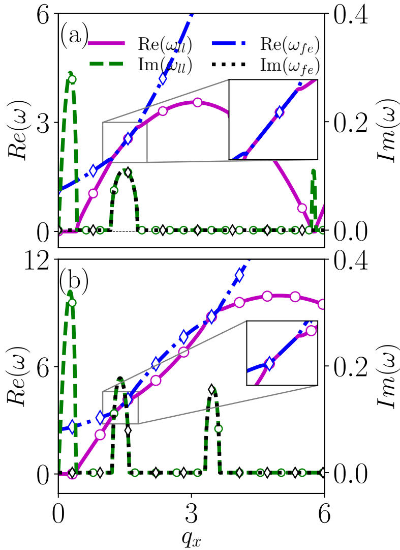
Figure 4.9: Excitation spectrum (a), and (b) for the coupling strengths, (k_L, \Omega) = (3.1, 1.17) and (5.0, 2.5) depict the low-lying and first-excited branches of the spectrum. The solid magenta line represents the Re(\omega_-) and the dashed green line represents the |Im(\omega_-)| which is low-lying branch of the spectrum, while the blue dash-dotted line represents Re(\omega_+) and black dotted line represents |Im(\omega_+)| corresponding to the first-excited branch of the spectrum, which obtained from Eq. 4.12. The eigenspectrum in (a, b) shows multiple instability bands as we obtained in 4.6(a1), however, (a) and (b) show one and two mode corresponding to no gap exists between the lower branch and first excited branch. Insets are for the better visualization of no gap mode between the lower and first excited state branch, the secondary y -axis scale is for representing the imaginary eigenfrequencies magnitudes.
