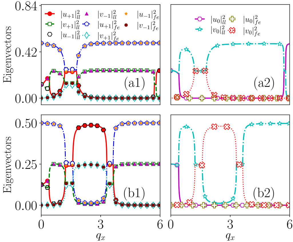
Figure 4.10: The eigenvectors top and bottom rows corresponding to Fig. 4.9(a), and Fig. 4.9(b), respectively. The eigenvectors represents as |u_{+1}|_{ll}^2 (red dot), |u_{-1}|_{ll}^2 (black hexagons), |u_0|_{ll}^2 (magenta hexagons), |v_0|_{ll}^2 (cyan open stars), |v_{+1}|_{ll}^2 (green open squares), and |v_{-1}|_{ll}^2 (magenta triangles). Whereas, |u_{+1}|_{fe}^2 (blue open pentagon), |u_{-1}|_{fe}^2 (orange stars), |u_0|_{fe}^2 (olive open plus), |v_0|_{fe}^2 (red open x with the dotted line), |v_{+1}|_{fe}^2 (cyan open diamond), and |v_{-1}|_{fe}^2 (maroon dots). We depict the +q_x , however, the eigenfrequencies and eigenvectors are symmetric about the axis. Here we found that the eigenvectors show the spin-like mode when the complex-frequency exhibits, the density-like mode when it is only real.
