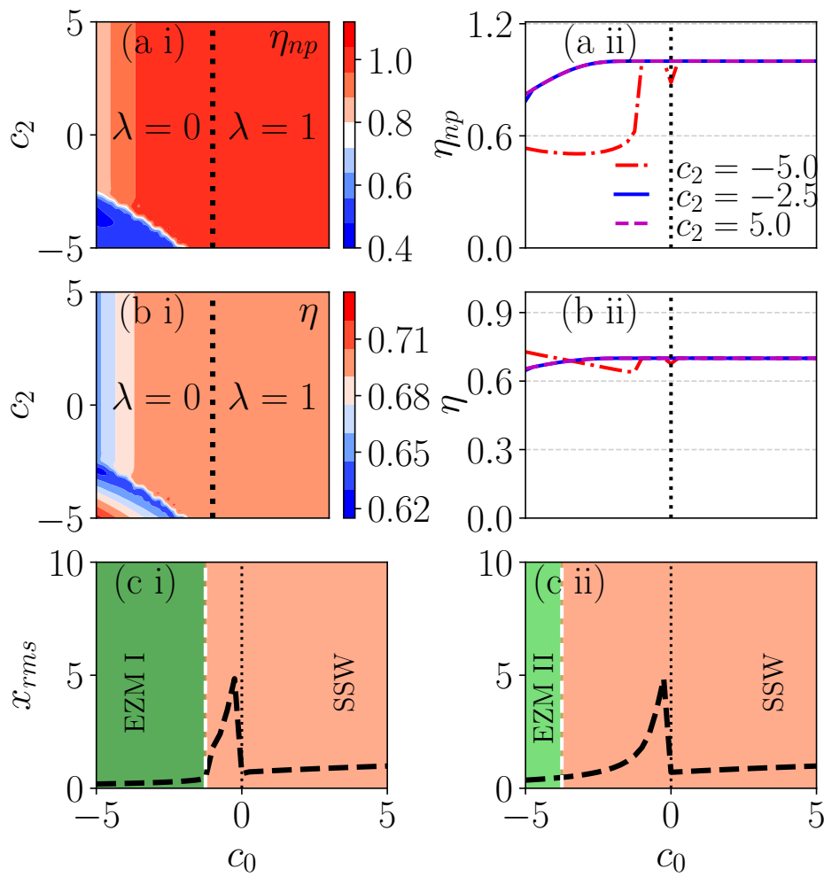
Figure 3.12: Miscibility parameters (a) \eta_{np} , and (b) \eta upon varying c_0 and keeping k_L = 3.0 and \Omega \sim 0 . In (a i) and (b i), c_0 and c_2 vary within the range [-5, 5] . (a ii) and (b ii) exhibit the \eta_{np} and \eta upon varying c_0 for c_2 = -5.0 (dashed-dotted red line), -2.5 (solid blue line), and 5.0 (dashed magenta line). In the bottom row, panels (c i) and (c ii) represent the root mean square ( x_{rms} ) size of the condensate for c_2 = -5.0 and 5.0 , respectively, which indicate different phases of the condensate. The color code represents different quantum phases: green represents the EZM I phase, limegreen represents the EZM II phase, and coral represents the SSW phase. The black dotted line separates untrapped ( c_0 < 0 ) and trapped ( c_0 \gtrsim 0 ) regimes of the condensate.
