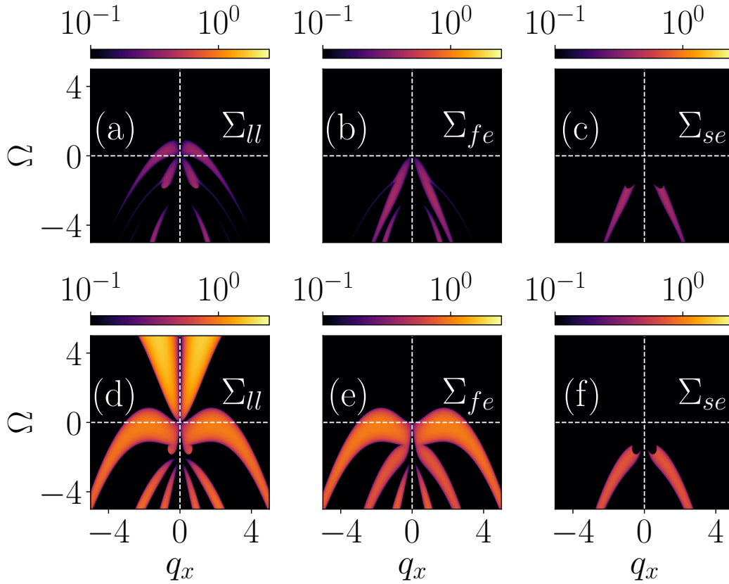
Figure 5.3: Pseudo color plot of the Modulational instability gain in \Omega - q_x phase plane for ferromagnetic interactions ( c_0 = 5.0 , and c_2 = -2.0 ) with (a-c) for k_L = 1 , and (d-f) for k_L = 4.0 . (a,d) represents \Sigma_{ll} \equiv |\text{Im}(\omega_{ll})| , (b,e) represents \Sigma_{fe} \equiv |\text{Im}(\omega_{fe})| and (c,f) for \Sigma_{se} \equiv |\text{Im}(\omega_{se})| low-lying, first-excited, and second-excited branches of the excitation spectrum. In (a), the primary band appears for \Omega > 0 following the relation k_L^2 = \Omega , while in (b) and (c), it appears only for \Omega < 0 , with a cutoff in (c), \Omega \approx -1.66 . Similar to the top row, the primary instability band in (d) appears for \Omega > 0 . In (d) and (e), the secondary and primary bands appear for \Omega > 0 different than the top row. In (f), single band instability appears for \Omega < 0 , following a cutoff value \Omega \approx -1.44 . The instability gain appears is not symmetric about \Omega and increases upon decreasing the \Omega . However, it shows symmetric behaviour about q_x .
