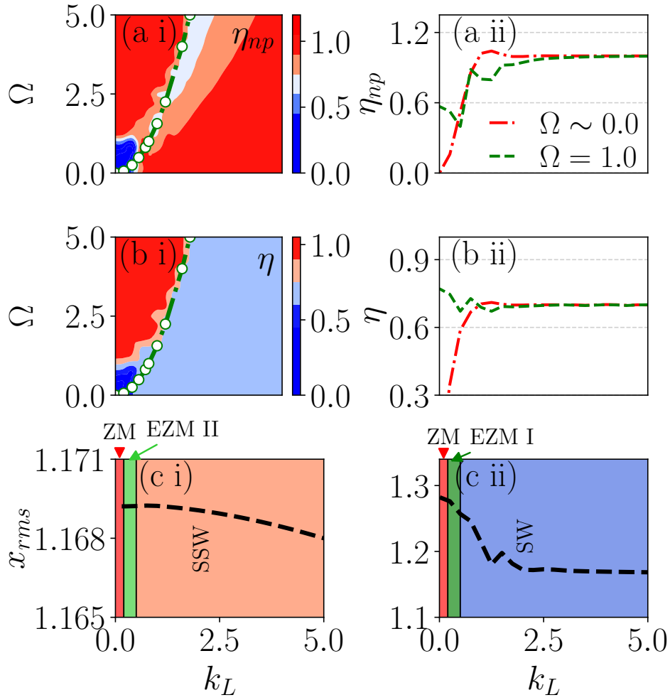
Figure 3.6: Miscibility parameters (a) \eta_{np} and (b) \eta for interaction strengths c_0 = 10 and c_2 = 5.0 . (a i) and (b i) show \eta_{np} and \eta as functions of spin-orbit coupling strength k_L in the range [0, 5] and Rabi coupling varies from small but finite values up to 5. The green line with white dots marks the critical relation k_L^2 \approx \Omega . Beyond this boundary ( k_L^2 > \Omega ), both \eta_{np} and \eta decrease. However, \eta_{np} exhibits a non-monotonic behavior—decreasing initially and rising again to near-maximum values. (a ii) and (b ii) display \eta_{np} and \eta as functions of k_L for fixed \Omega \sim 0.0 (dash-dotted red line) and \Omega = 1.0 (dashed green line). Panels (c i) and (c ii) show the root-mean-square condensate size x_{rms} versus k_L for \Omega \sim 0.0 and \Omega = 1.0 , respectively. The background color represents distinct quantum phases: red (ZM), green (EZM I), limegreen (EZM II), blue (SW), and coral (SSW).
