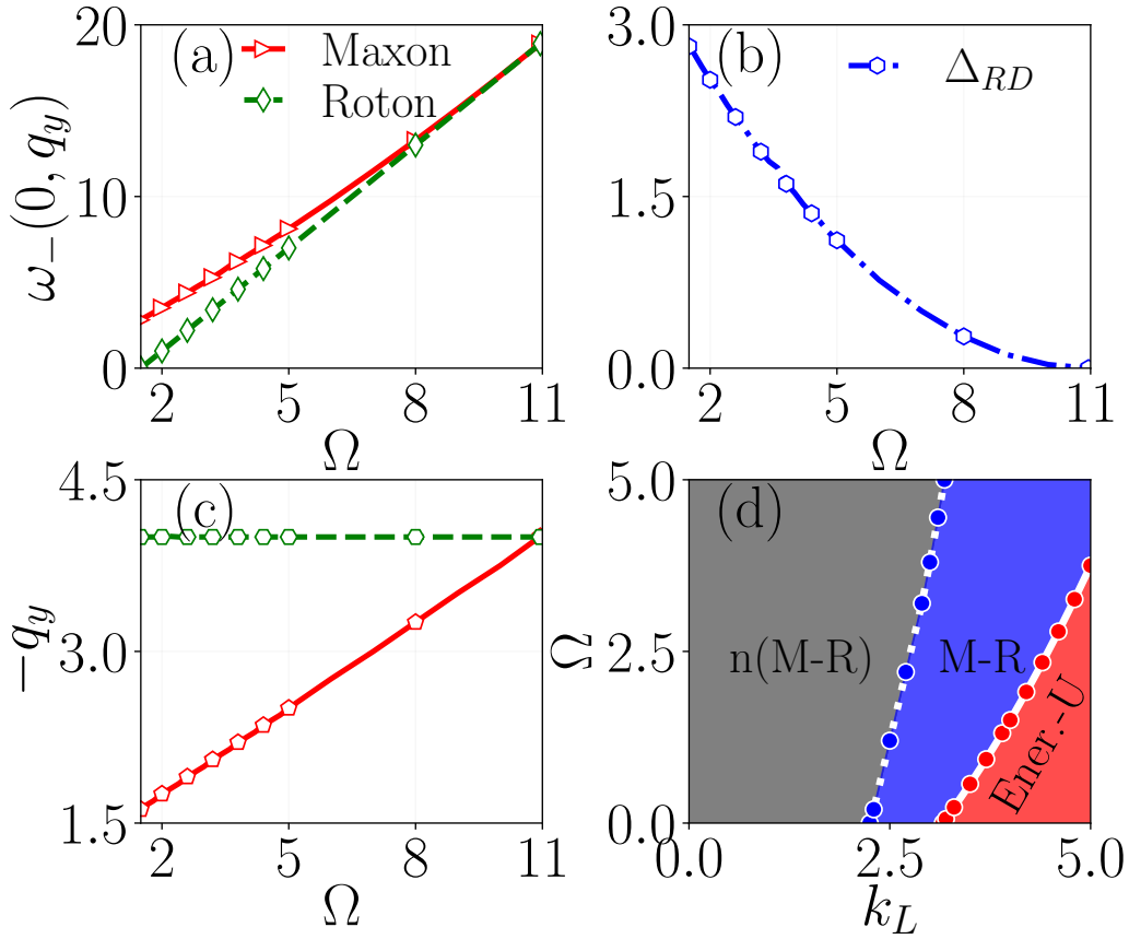
Figure 6.7: Variation of roton-maxon modes for ferromagnetic interaction ( c_0 = 50 , c_2 = -2.5 ). Panels (a-c) show the results obtained for k_L = 4.0 as the Rabi coupling is varied. Panel (a) displays the evolution of the maxon (red open right triangles) and roton (green open diamonds) modes, while panel (b) shows the corresponding decay of the roton depth \Delta_{RD} (blue open hexagons). Panel (c) illustrates quasi-momentum positions of the maxon (red open pentagon) and roton (green open hexagons) modes along the q_y direction. Panel (d) presents the phase diagram in the k_L - \Omega plane at q_x = 0.0 , with gray, blue, and red regions indicating the absence of maxon-roton modes n(M-R) , the presence of maxon-roton modes (M-R), and energetic instability (Ener.-U), respectively, along the q_y direction.
