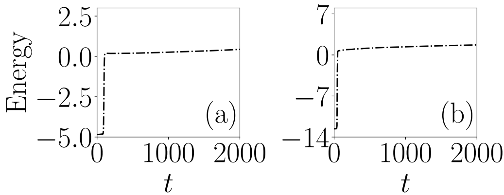
Figure 4.12: (a) and (b) depict the total energy of the condensate for the dynamical evolution for the Fig. 4.11. Following the quenching of trap strength, the condensate exhibits temporal variation in the energy during the evolution, followed by a steady behaviour at later times.
