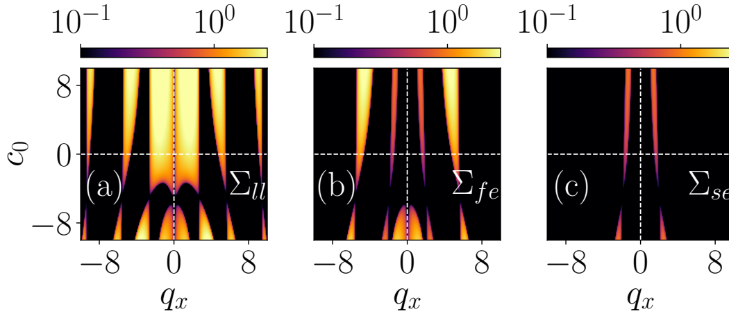
Figure 5.10: MI of antiferromagnetic interaction ( c_2 = 5.0 ) in c_0 - q_x phase for (a-c) k_L = 4.5, \Omega = 1.0 . The pseudo color bar is similar to Fig. 5.3. Multi-band instability in low-lying and first-excited branches and single-band instability in the second-excited branch of eigenspectrum increases upon increasing the c_0 and symmetry arguments are similar to figure 5.9.
