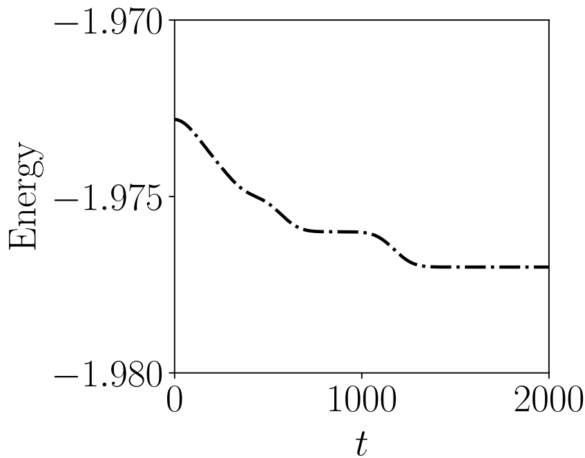
Figure 4.5: Energy variation in the time evolution for the stable region I. The parameter values considered in this figure are similar to Fig. 4.3. During time evolution, the condensate exhibits temporal variation of the energy and further shows stable behaviour.
