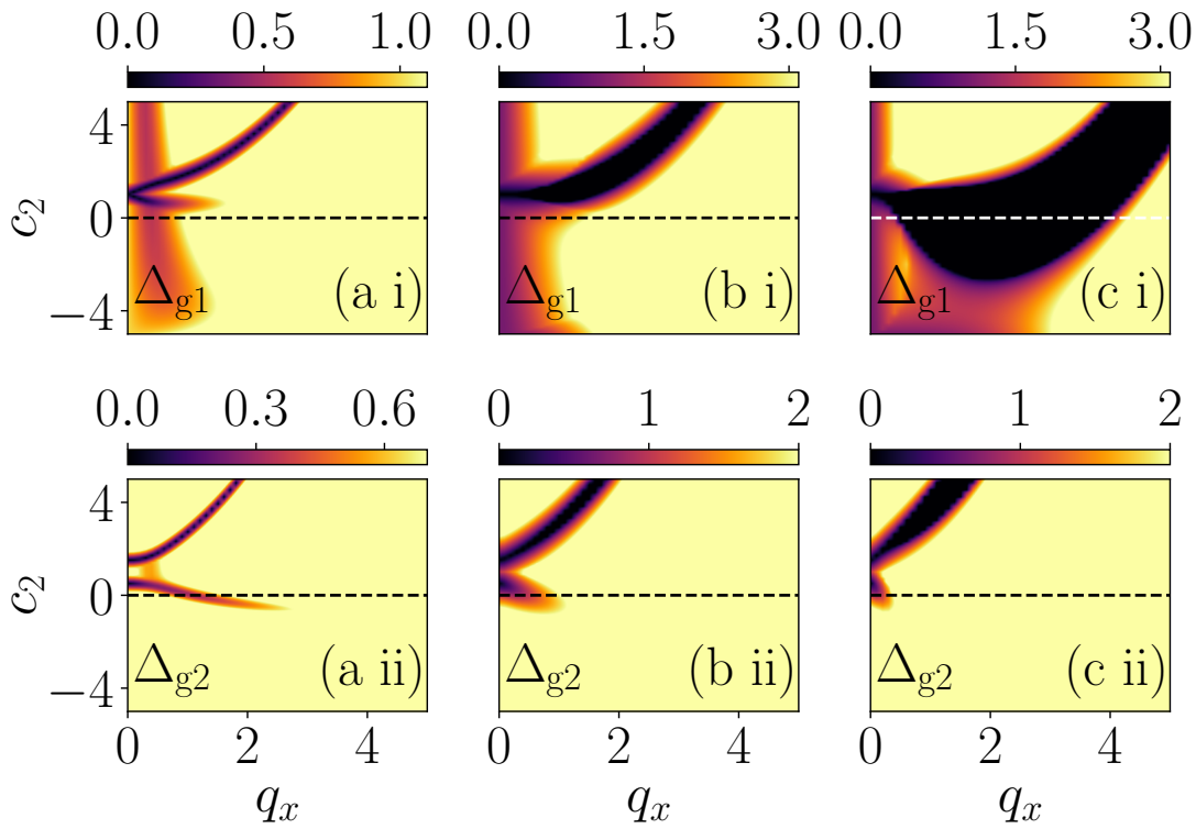
Figure 5.13: Pseudo color representation of the change in band gap \Delta_{g1} = \text{Re}(\omega_{fe}) - \text{Re}(\omega_{ll}) and \Delta_{g2} = \text{Re}(\omega_{se}) - \text{Re}(\omega_{fe}) for different k_L in c_2 - q_x plane by keeping \Omega = 1.0 , and c_0 = 5.0 . (a i, a ii) for k_L = 0.5 , (b i, b ii) for k_L = 2.0 and (c i, c ii) for k_L = 4.5 . For (a i, b i), the band gap \Delta_{g1} closes for positive c_2 > 0 (antiferromagnetic interaction). However, in (c i), it closes for both antiferromagnetic ( c_2 > 0 ) and ferromagnetic ( c_2 < 0 ) interactions. In (a ii - c ii), the band gap \Delta_{g2} closes for antiferromagnetic interactions only ( c_2 > 0 ).
