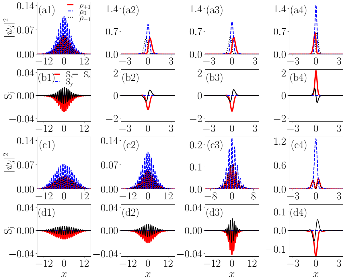
Figure 3.7: Ground state density profiles of |\psi_{+1}|^2 (solid red line), |\psi_0|^2 (dashed blue line), and |\psi_{-1}|^2 (dotted black line) in panels (a) and (c), and corresponding spin-density vector components S_x (solid red line), S_y (dashed blue line), and S_z (thin black line) in panels (b) and (d), for k_L = 3.0 and \Omega = 1.0 . Panels (a, b) correspond to c_2 = -5.0 , and panels (c, d) to c_2 = 5.0 . In each case, the density-density interaction c_0 varies as -0.25 , -0.50 , -1.0 , and -5.0 from left to right. The appearance of multipeak structures in S_x and oscillations in S_z indicates the SW phase, while a single peak in S_x with finite S_z signifies the EZM I phase. A transition from the SW to EZM I phase occurs with increasing |c_0| , for both c_2 < 0 and c_2 > 0 . As c_0 < 0 in all cases, no external trapping potential is applied.
