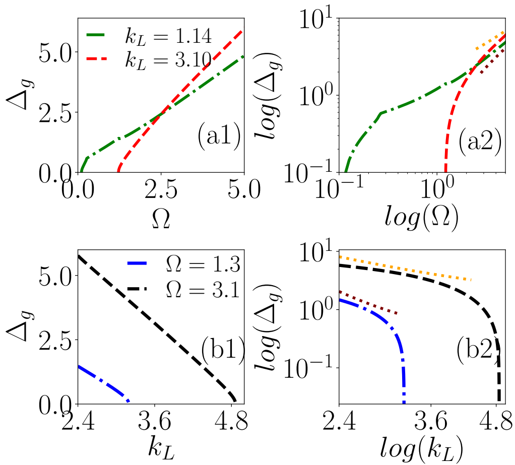
Figure 4.16: Variation of band gap \Delta_g between negative and positive branches of the spectrum. (a1) For the fixed value SO coupling strength upon variation of Rabi coupling strength, vice versa in (b1). In (a1), the dash-dotted green and the dashed red lines represent gap calculation for k_L = 1.14 and k_L = 3.10 , respectively. In (b1), the dash-dotted blue and the dashed black lines represent gap calculation for \Omega = 1.3 and \Omega = 3.1 , respectively. The interaction parameter strength are c_0 = 0.5 , and c_2 = -0.1 . (a2) and (b2) are the logarithmic scale plots corresponding to (a1) and (b1), respectively. Further, in (a2) and (b2) the maroon (orange) dotted lines represent the fitting curve \Delta_g = a\Omega^b with the parameters a = 0.9811, b = 0.9974 , ( a = 1.0825, b = 1.0258 ), and a = 126.2992, b = -4.9568 , ( a = 46.4438, b = -2.2146 ), respectively.
