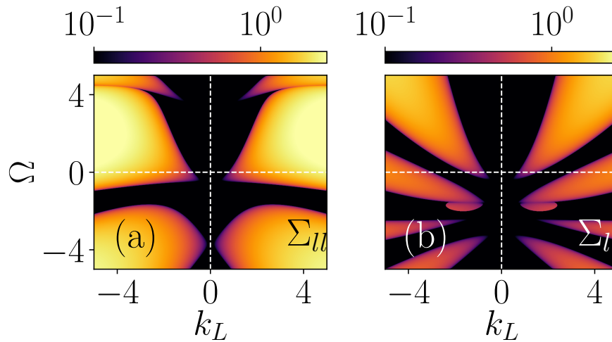
Figure 5.8: Pseudo color representation of the MI gain for \Sigma_{ll} \equiv |\text{Im}(\omega_{ll})| in k_L - \Omega phase plane for (a) (c_0, c_2) = (5, 5) and (b) (c_0, c_2) = (5, -2) at quasi-momentum q_x = 1 . Multi-band instability appears in each case, which increases upon increasing the k_L . The instability bands show symmetric behaviour about k_L , however, it is not symmetric with the variation in \Omega .
