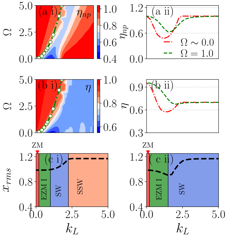
Figure 3.3: Miscibility parameters (a) \eta_{np} and (b) \eta for interaction strengths c_0 = 10 and c_2 = -5.0 . The top rows of (a) and (b) show pseudo color representation of \eta_{np} and \eta as a function of k_L in the range [0, 5] and \Omega varies from small but finite values up to 5. The green line with white dots marks the critical relation k_L^2 \approx \Omega , beyond which both \eta_{np} and \eta begin to decrease. \eta_{np} shows decreasing trend for intermediate values of k_L and then rises again. (a ii) and (b ii) show the \eta_{np} and \eta as a function of k_L for \Omega \sim 0.0 (dashed-dotted red line), and 1.0 (dashed green line). Panels (c i) and (c ii) show the root mean square size ( x_{rms} ) as a function of k_L for \Omega \sim 0.0 and \Omega = 1.0 , respectively. Background color shading indicates distinct quantum phases: red (ZM), green (EZM I), blue (SW), and coral (SSW).
