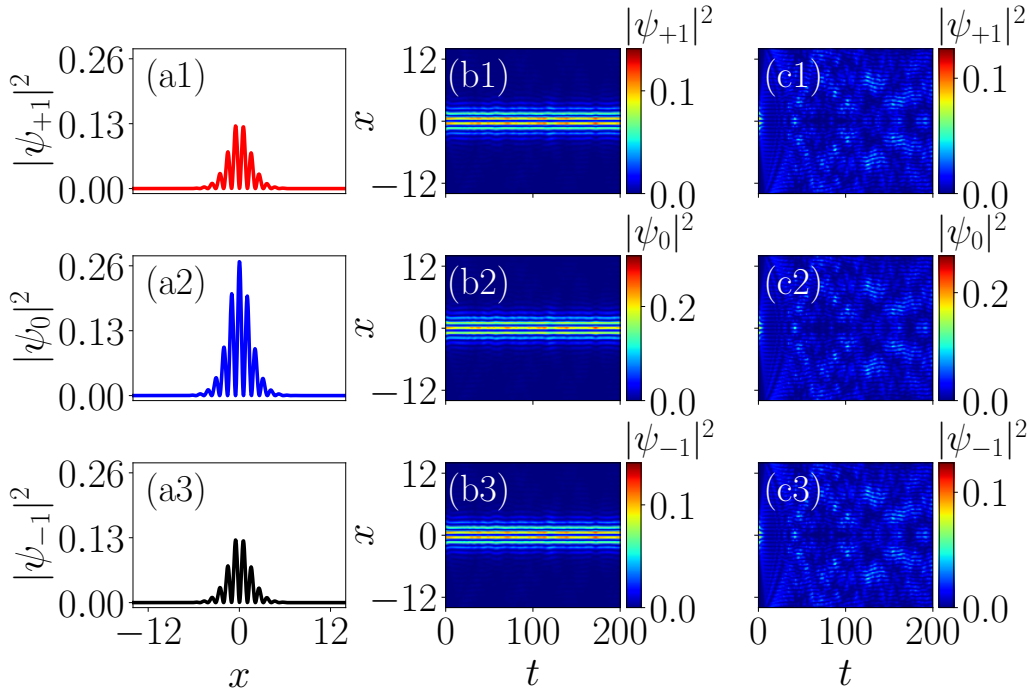
Figure 3.15: Ground state density profile (a1-a3) for m_F = +1, 0, -1 , respectively, with ( k_L = 3.0, \Omega \sim 0.0 ). The interaction strengths are c_0 = -1.0 , and c_2 = 5.0 . The condensate is in the SSW phase. Panels (b1-b3) and (c1-c3) exhibit dynamics of the ground state profile in the x-t plane upon quenching the SO coupling strength k_L = 3.0 \rightarrow 3.20 and k_L = 3.0 \rightarrow 4.0 , respectively. The SO coupling is quenched at t = 0 units. The strong quench of the SO coupling strength leads to the emergence of complex patterns.
