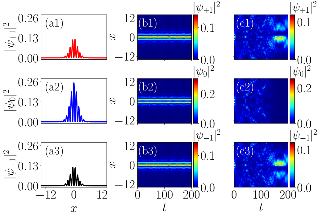
Figure 3.14: Ground state density profile (a1-a3) for m_F = +1, 0, -1 , respectively, with (k_L, \Omega) = (3.0, 1.0) . The interaction strengths are c_0 = -1.0 , and c_2 = 5.0 . The condensate is in the SW phase. Panels (b1-b3) and (c1-c3) depict the time evolution of the initially prepared density profile in the x-t plane upon quenching the SO coupling strength k_L = 3.0 \rightarrow 3.20 and k_L = 3.0 \rightarrow 4.0 , respectively. The SO coupling is quenched at t = 0 units. For a stronger quench of the Rabi coupling strength, the condensate fragments into small domains, forming a complex pattern, and the zeroth component disappears at a later time unit.
