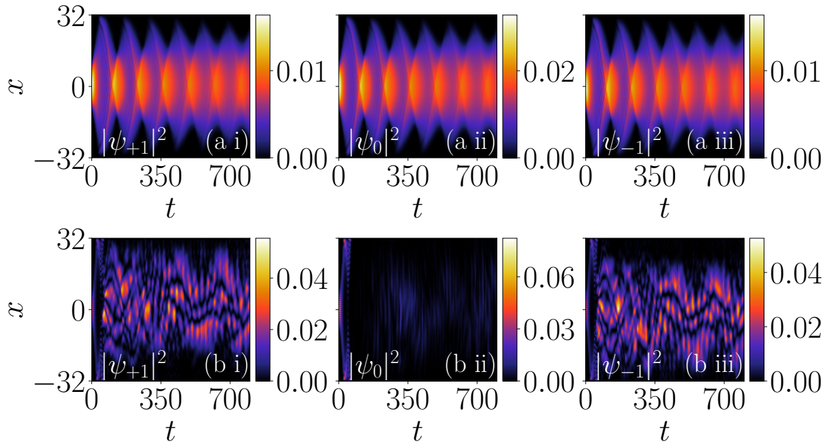
Figure 5.15: Dynamical evolution of the condensate in x-t plane for |\psi_{+1}|^2 , |\psi_0|^2 , |\psi_{-1}|^2 components of the condensate for (top row) k_L = 0.5, \Omega = 1.0 and (bottom row) k_L = 4.5, \Omega = 1.0 , by quenching the trap strength to one-third of its initial value. The interaction strengths are c_0 = 5.0 , and c_2 = 5.0 . In the PW phase, the density of the condensate shows stable breather-like dynamics. The SW phase holds its shape in the beginning, further |\psi_{\pm 1}|^2 components fragments in several small domains, and zeroth components start diminishing, confirming the dynamical instability of the condensate.
