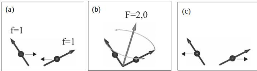
Figure 1.4: Intuitive picture showing the process of atomic interactions in spin-1 bosons. (a) Two bosons of hyperfine spin f = 1 approach each other. (b) They couple together and form a total spin F = 0, 2 ; precess around the total spin F during the collision. (c) Two bosons are separated from each other after the collision is finished. The figure is adopted from the Ref. [35].
