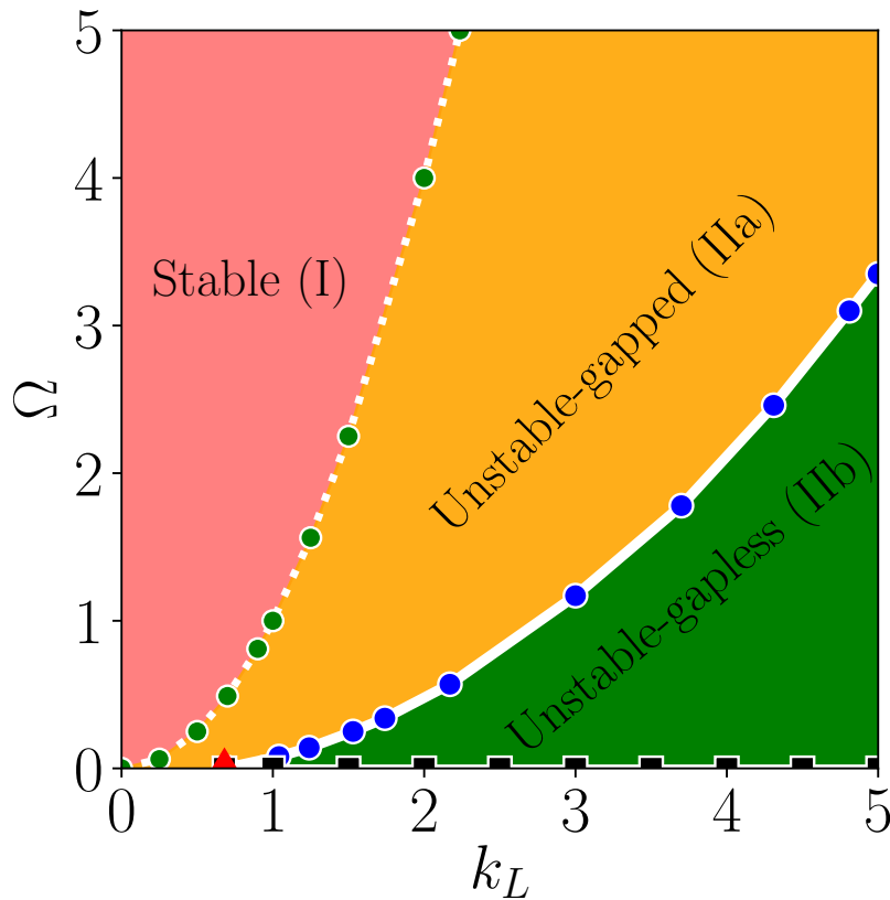
Figure 4.2: Stability phase diagram in the k_L - \Omega plane for the interaction parameter c_0 = 0.5 , c_2 = -0.1 which is being considered for all the simulation runs. Based on the different characteristics of the eigenspectrum and ground state, the phase diagram is divided into regions I, IIa, IIb, and III. While Region I is stable, regions IIa, IIb, and III are unstable. The dotted white line along with green dots represent the \Omega = k_L^2 curve that separates region I from IIa. Blue dots with a white solid line representing \Omega \approx 0.1365k_L^2 - 0.0686 separates the regions IIa and IIb. The horizontal line with a filled half square for \Omega \sim 0 denotes the region III after the cutoff, k_L^c = 0.68 , which is a tricritical point for regions IIa-IIb-III, indicated as a red triangle.
