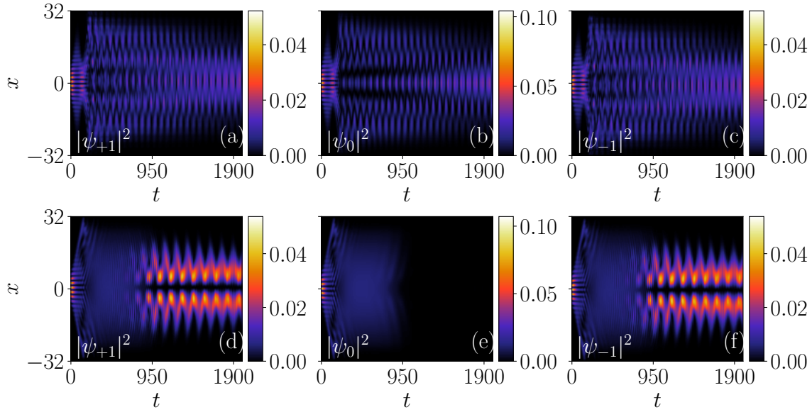
Figure 4.7: Dynamics: (a-c) and (d-f) depict temporal evolution of stationary state density profile of |\psi_{+1}|^2 , |\psi_0|^2 , and |\psi_{-1}|^2 for (k_L, \Omega) : top row (2.0, 2.0) and bottom row (2.35, 4.0), respectively. The density profile holds stripe wave behavior in both cases for t < 150 , and t < 180 for the top and bottom row, respectively. Further, it gets fragmented into several small domains. This behavior signifies the change in shape and amplitude of the density profile, where the bottom row 0-th component gets diminished, whereas the \pm 1 components gained the density.
