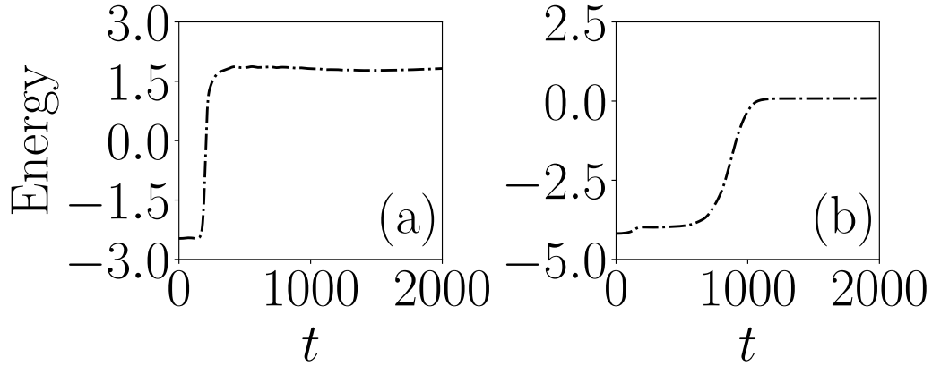
Figure 4.8: (a) and (b) represent the total energy of the condensate for the density evolution in Fig. 4.7. In both cases, the energy of the condensate increases at the beginning of dynamical evolution, but finally shows well-settled stable behavior; such a sudden change happened due to the external perturbation.
