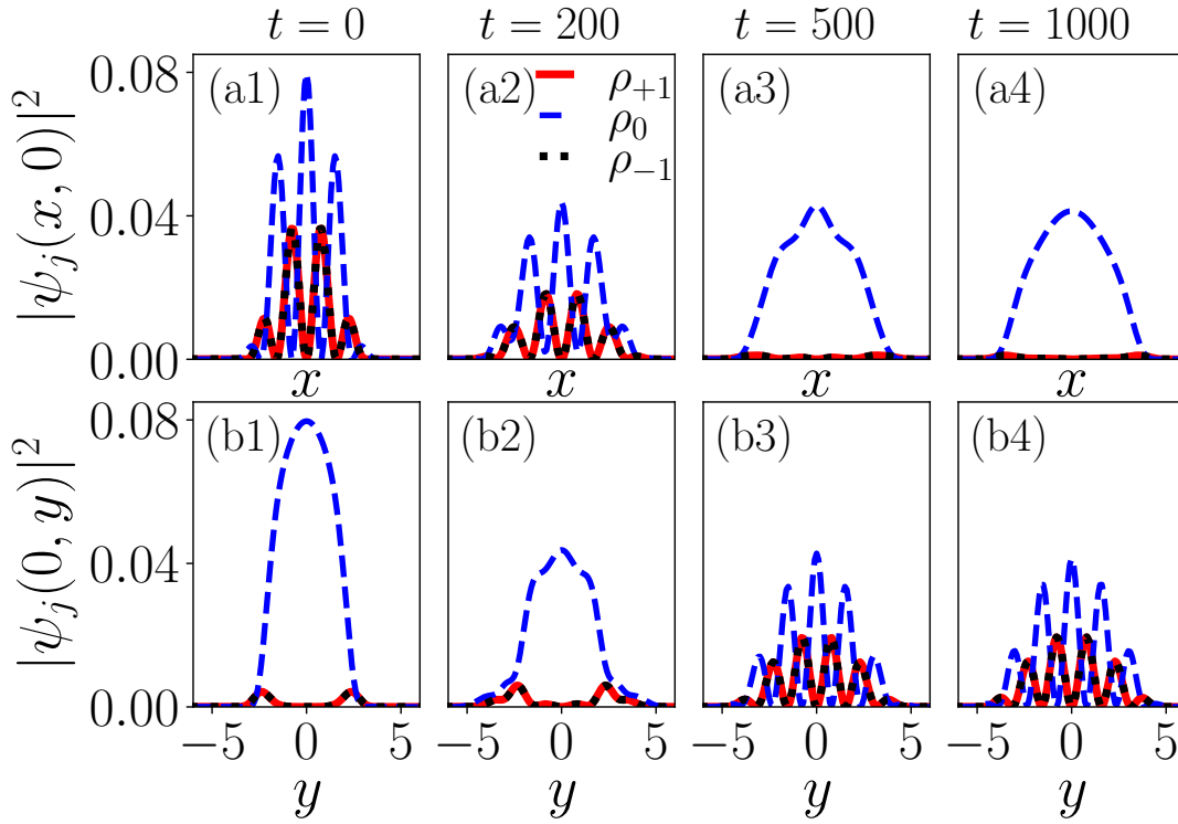
Figure 6.17: (a1, b1) Stationary state density profiles. (a2–a4, b2–b4) Density profiles at evolution times t = 200, 500 , and 1000 (arb. units). The top row shows the density along the spatial x -direction at y = 0 , and the bottom row shows the density along the y -direction at x = 0 . Coupling parameters and interaction strengths are the same as in Fig. 6.16. The solid red line represents |\psi_{+1}|^2 , the dashed blue line |\psi_0|^2 , and the dotted black line |\psi_{-1}|^2 .
