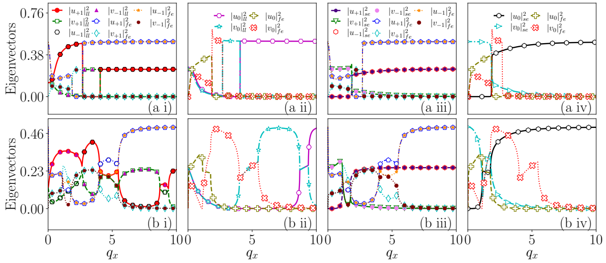
Figure 5.5: Eigenvectors corresponding to Figs. 5.4(a) and (b), in (a) and (b), respectively. (a i, a ii), and (b i, b ii) represents eigenvectors of the low-lying and first-excited branch, while (a iii, a iv) and (b iii, b iv) for the second-excited and first-excited branch of the eigenspectrum. The eigenvectors of the low-lying branch are given as |u_{+1}|_{ll}^2 (red dot), |u_{-1}|_{ll}^2 (black hexagons), |u_0|_{ll}^2 (magenta hexagons), |v_0|_{ll}^2 (cyan open stars), |v_{+1}|_{ll}^2 (green open squares), and |v_{-1}|_{ll}^2 (magenta triangles). For the first-excited branch, |u_{+1}|_{fe}^2 (blue open pentagon), |u_{-1}|_{fe}^2 (orange stars), |u_0|_{fe}^2 (olive open plus), |v_0|_{fe}^2 (red open x with the dotted line), |v_{+1}|_{fe}^2 (cyan open diamond), and |v_{-1}|_{fe}^2 (maroon dots). The eigenvectors of the second-excited branch are given as |u_{+1}|_{se}^2 (indigo dot), |u_{-1}|_{se}^2 (red hexagons), |u_0|_{se}^2 (black hexagons), |v_0|_{se}^2 (cyan triangle left), |v_{+1}|_{se}^2 (green open triangle down), and |v_{-1}|_{se}^2 (violet dots). (a i - a iv) depict in-phase behaviour (density-like mode) with the occurrence of flip at the point of stable avoided crossing between \omega_{ll} - \omega_{fe} , and \omega_{se} - \omega_{fe} . (b i, b iii) exhibit the out-of-phase behaviour (spin-like mode). At the point of UAC, eigenvectors are out-of-phase among the branches. However, (b ii, b iv) only depict density-like mode.
