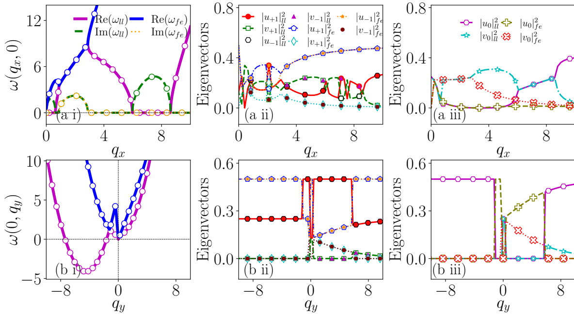
Figure 6.9: Eigenspectra and corresponding eigenvectors for the spinor condensate are shown, with the top (bottom) row corresponding to quasi-momentum along q_x ( q_y ) for (k_L, \Omega) = (4.5, 0.5) , and interaction strengths c_0 = 50.0 , c_2 = -2.5 . Panels (a i) and (b i) display the eigenspectra, with \text{Re}(\omega) shown as solid lines and |\text{Im}(\omega)| as dashed or dotted lines. The eigenvector components for the low-lying and first-excited branches are shown in panels (a ii, a iii) and (b ii, b iii), respectively. Multi-band instability appears in the low-lying branch, single-band instability in the first-excited branch arises from avoided crossings along q_x , and negative eigenfrequencies are observed along q_y .
