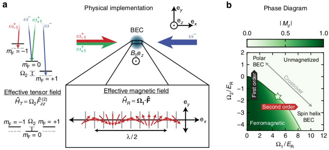
Figure 1.7: (a) Schematic and level diagram. The |-1\rangle \leftrightarrow |0\rangle and |0\rangle \leftrightarrow |+1\rangle transitions of the F = 1 ground state of ^{87}\text{Rb} were independently Raman coupled, giving experimental control of \Omega_1 and \Omega_2 . (b) Phase diagram. The ferromagnetic order parameter is plotted against \Omega_2 and \Omega_1 . The dashed (solid) red curve denotes the first-order (second-order) transition from the magnetized phase. This figure is taken from Ref. [10].
