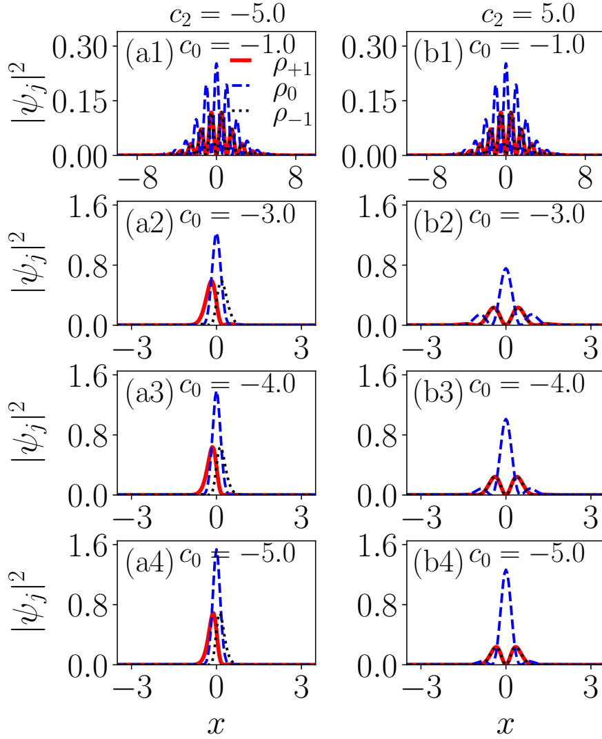
Figure 3.10: Ground state density profile |\psi_{+1}|^2 (solid red line), |\psi_0|^2 (dashed blue line), and |\psi_{-1}|^2 (dotted black line) upon varying c_0 , keeping k_L = 3.0 and \Omega \sim 0.0 with (a) c_2 = -5.0 , and (b) c_2 = 5.0 . The density-density interaction strength varies as c_0 = -1.0, -3.0, -4.0 , and -5.0 in columns from top to bottom. A phase transition takes place from the SSW phase to the EZM I phase and EZM II phase upon increasing the magnitude of c_0 for c_2 < 0 and c_2 > 0 , respectively. Since c_0 < 0 , no external trapping is required.
