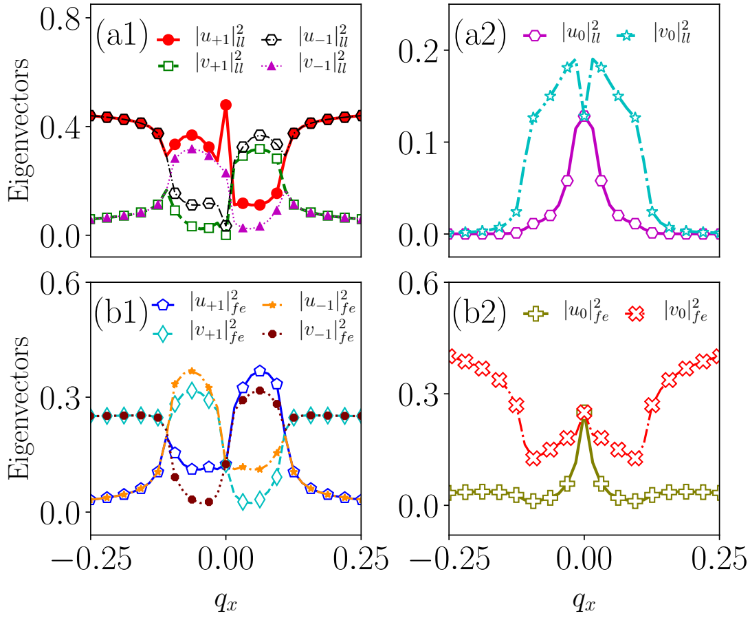
Figure 4.14: Eigenvectors top and bottom rows are corresponding to the Fig. 4.13(a) and, Fig. 4.13(b) respectively. The label representation is similar to the Fig. 4.10. In this region, both low-lying and the first excited state assume the value \omega = 0 for q_x = 0 with eigenvectors are in-phase with the low-lying and first-excited states, which indicates the existence of the phonon mode for these branches.
