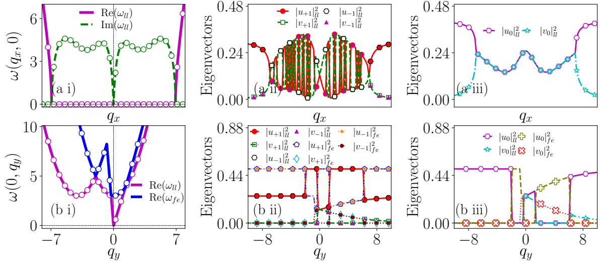
Figure 6.6: Eigenvalue spectra [(a i), (b i)] and corresponding eigenvectors [(a ii, a iii) and (b ii, b iii)] for k_L = 4.0 and \Omega = 3.0 with interaction strengths c_0 = 50.0 and c_2 = -2.5 , shown along the quasi-momentum directions q_x and q_y , respectively. Line styles and symbols follow the conventions of Fig. 6.3. A single-band instability appears in the low-lying branch along the q_x direction, while a roton-maxon-like feature develops in the low-lying branch along the q_y direction.
