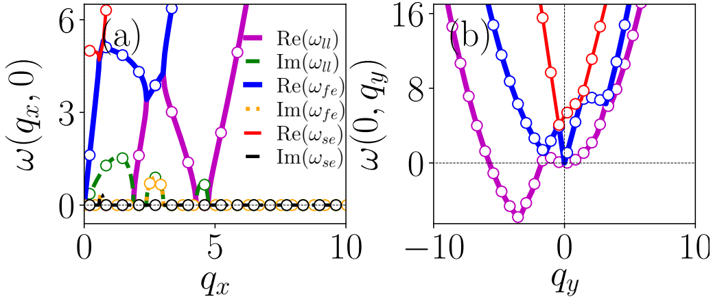
Figure 6.14: Collective excitation spectrum as a function of (a) quasi-momentum q_x and (b) quasi-momentum q_y . Parameters are SO coupling strength k_L = 2.0 , Rabi frequency \Omega = 0.0 , and interaction strengths c_0 = 50, c_2 = 2.5 . Solid magenta, solid blue, and thin red lines represent \text{Re}(\omega_{ll}) , \text{Re}(\omega_{fe}) , and \text{Re}(\omega_{se}) , respectively; dashed green, dotted orange, and dash-dotted black lines show the corresponding magnitude of the imaginary part |\text{Im}(\omega)| . A multiband instability with a roton minimum appears along q_x , while negative excitation frequencies are observed along q_y .
