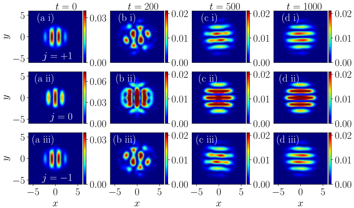
Figure 6.16: Pseudocolor plots of the condensate density for the spin-1 system. Plot of (a) the stationary state density profile exhibiting a superstripe phase and (b–d) density profiles during dynamical evolution at times t = 200, 500 , and 1000 (in arbitrary units), respectively. In each subfigure, columns (i), (ii), and (iii) correspond to the m_F = +1, 0 , and -1 spinor components. The system parameters are fixed at k_L = 2.0, \Omega = 0.0 , and interaction strengths c_0 = 50, c_2 = 2.5 .
