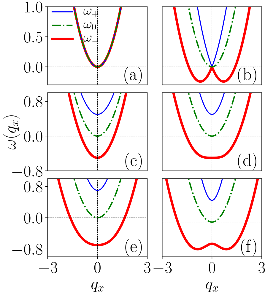
Figure 4.1: Single-particle energy spectrum in momentum space for the different set of SO and Rabi coupling strengths (k_L, \Omega) : (a)-(f): (0, 0) , (0.7, 0) , (0, 0.5) , (0.7, 0.5) , (0.7, 0.7) , (1.0, 0.5) . The thick-solid-red, dash-dotted green line and thin-solid-blue line represent the energy eigenspectrum for \{-1, 0, +1\} components of the spin, respectively. Varying the coupling parameters lead to the changes in the eigenspectrum of different components, where \omega_- , only having the lowest minimum for \Omega > k_L^2 , whereas \Omega < k_L^2 , the \omega_- exhibits double minima appearance of plane-wave phase, indicating the presence of stripe phase.
