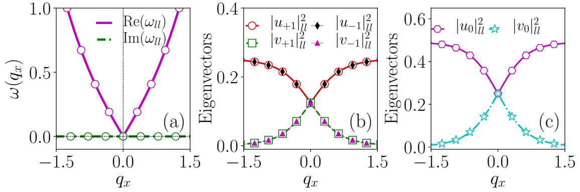
Figure 4.3: Excitation spectrum (a) and eigenvectors (b) and (c) for the coupling parameters k_L = 0.5 , \Omega = 2.0 . (a) solid magenta line represents \text{Re}(\omega_{II}) , and dashed-dotted green line represents the |\text{Im}(\omega_{II})| , here solid and dash-dotted lines are the analytical results of BdG Eq. 4.12 and open circles are numerical results obtained by solving Eq. 4.9. In the eigenvectors, |u_{+1}|^2 (red open circles), |u_{-1}|^2 (black diamonds), |u_0|^2 (magenta open hexagons), |v_0|^2 (cyan open stars), |v_{+1}|^2 (green open squares), and |v_{-1}|^2 (magenta triangles), (b-c) the eigenvectors corresponding to eigenspectrum has shown, which we obtained by solving Eq. 4.9 numerically. The first column of the figure shows the presence of phonon mode in the eigenspectrum. Also, it has no negative or complex eigenfrequency thus, it is energetically and dynamically stable.
