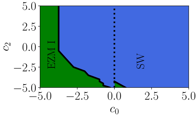
Figure 3.8: Ground state phase diagram in the c_0 - c_2 plane for fixed k_L = 3.0 and \Omega = 1.0 . The black dotted line separates the trapless ( c_0 < 0 ) and trapped ( c_0 \gtrsim 0 ) regimes. Different quantum phases are indicated by color: green denotes the EZM I phase and blue denotes the SW phase. For considered parameter (k_L, \Omega) = (3.0, 1.0) , the system resides in the SW phase under weak or repulsive interaction strengths, while the higher attractive strength of both c_0 and c_2 drives a transition into the EZM I phase.
